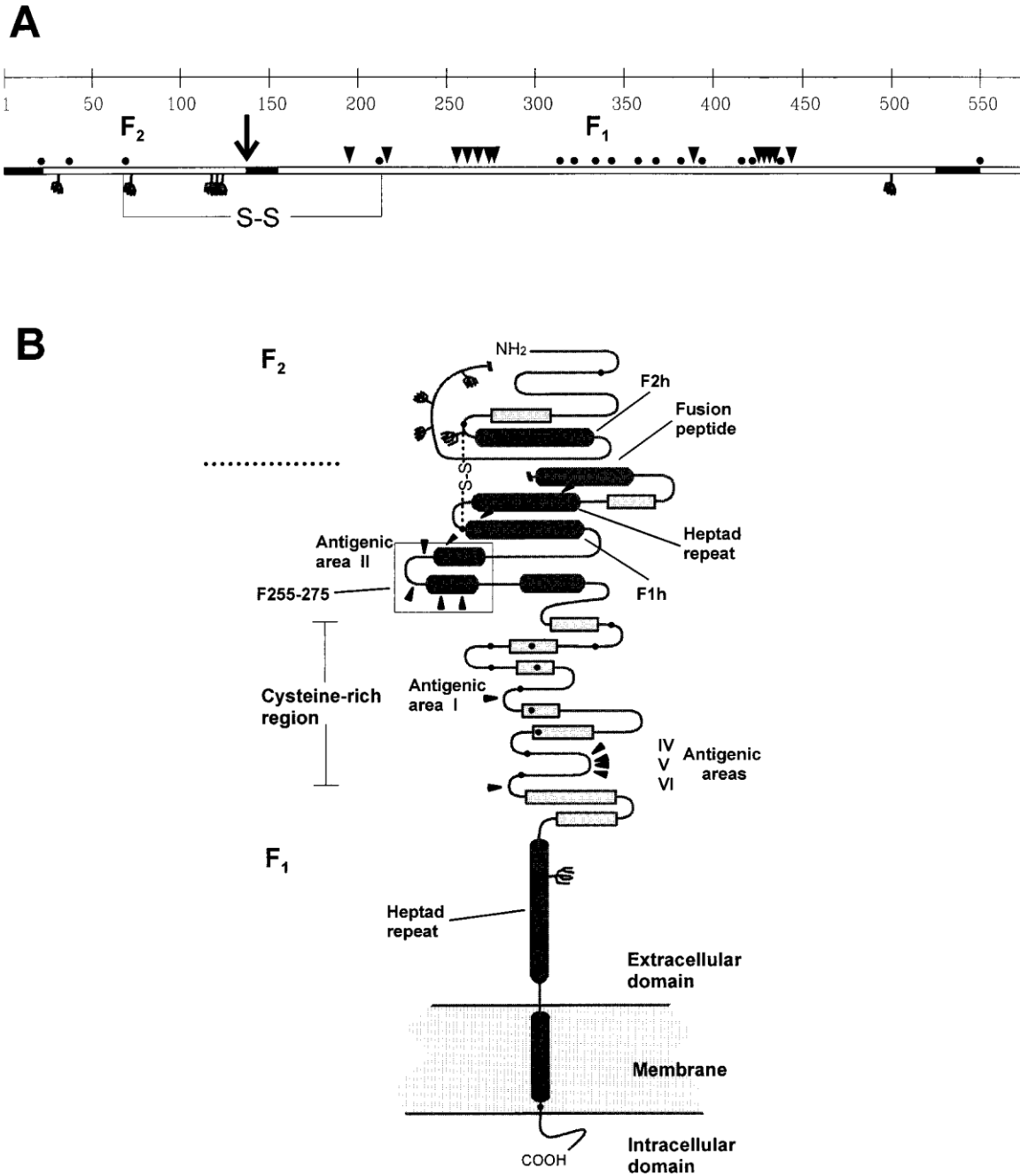
FIG. 4. Prediction of secondary-structure motifs of the F protein. (A) Linear diagram of the F protein polypeptide of the Long strain (22) showing cysteine residues (—), potential N-glycosylation sites (○), site of proteolytic processing (∇), amino acid changes in escape mutants reported here and in previous publications (◊) and hydrophobic regions (■). S-S, disulfide bridge. (B) Predicted secondary-structure elements of the F protein: \alpha -helices (cylinders), \beta -sheets (rectangles), loops (turns). Other symbols are as explained for panel A. The segment between residues 255 and 275 (F255-275), predicted to fold in a helix-loop-helix structure, is boxed. F1h and F2h, amphipathic \alpha -helices in the F1 and F2 chains, respectively. The diagram is not drawn to scale. The predictions were made with published sequences of pneumovirus F proteins and by using the following methods available on Worldwide Web servers: the PHD method (33, 34) ( http://www.embl-heidelberg.de/predictprotein/predictprotei.html ), the DSC method (18) ( http://bonsai.lif.icnt.uk/bmm/dsc_form_align.html ), and the PREDATOR method (11) ( http://embl-heidelberg.de/predator/predator_info.html ), which use multiple aligned protein sequences as input to estimate the probability of secondary-structure motifs and solvent accessibility; and the SOPMA method (13) ( http://www.ibcp.fr/serv_pred.html ), the nnPREDICT method (19) ( http://www.cmpharm.ucsf.edu/nomi/nnpredict.html ), and the PSA method (38) ( http://bmerc-www-bu.edu/psa/ ), which use single protein sequences as input. The final secondary-structure model was a consensus of the information obtained by the different methods. Details of the prediction studies are available from the authors upon request.
