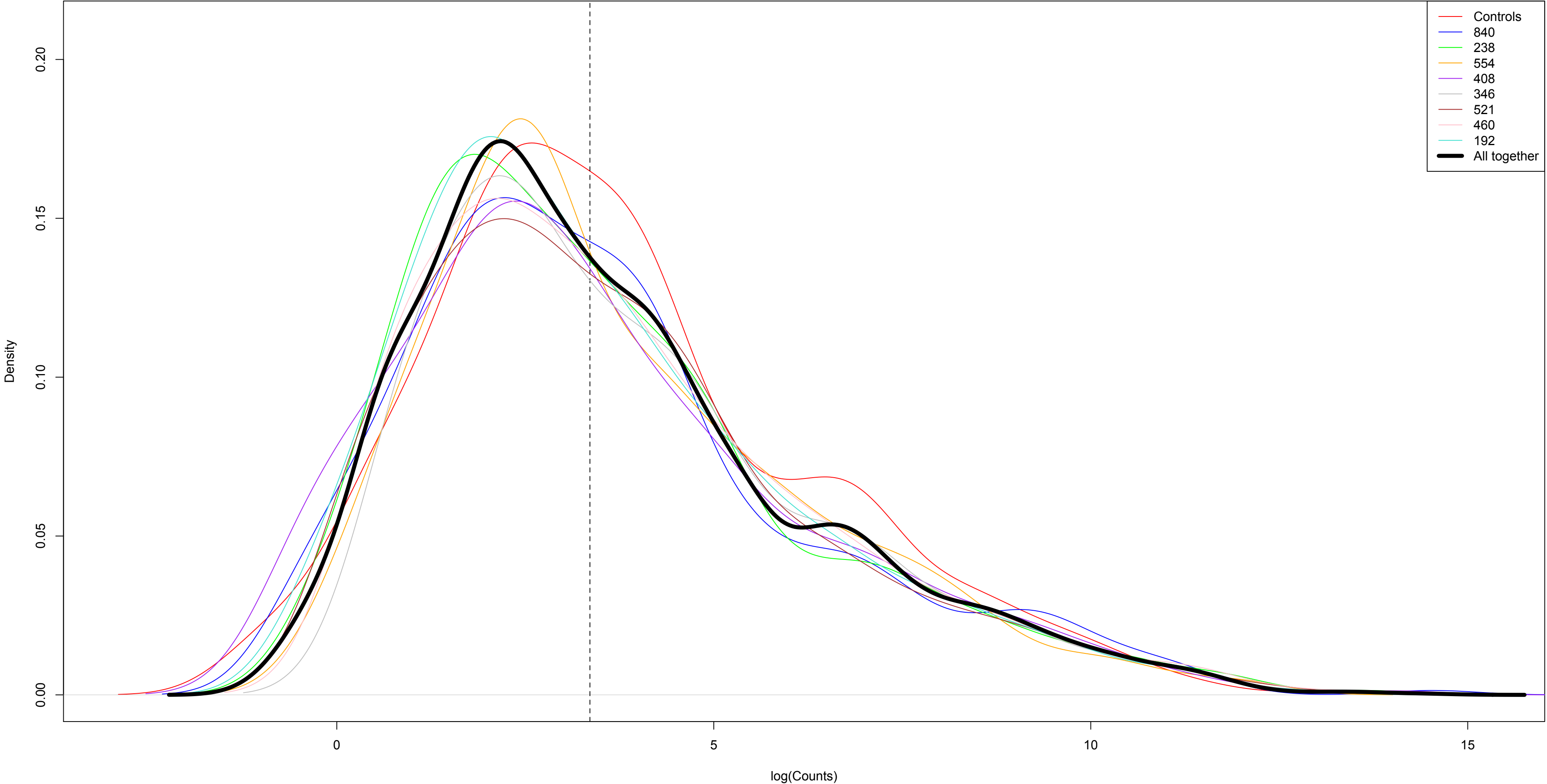
Fig S2. Gaussian Kernel Density Plot of the read counts for the miRNAs deregulated in any sample. Black dashed line represents the median value (28.70) of the miRNA read counts of all the samples and red line represents the mean value of the controls read counts.
