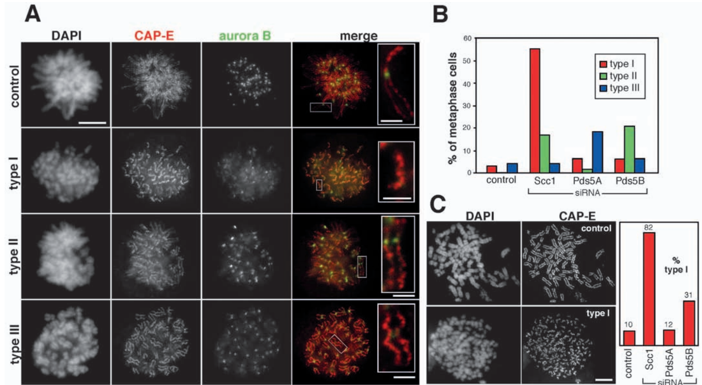
Fig. 4. Cohesion defects in cells with reduced levels of cohesin or Pds5 proteins. (A) HeLa cells grown on coverslips that had been transfected with no siRNA (control) or with siRNAs specific to Scc1, Pds5A or Pds5B were incubated in 60 mM KCl for 30 minutes, fixed and stained with DAPI, anti-condensin (CAP-E/Smc2) and anti-aurora B. In the 'merge' panels, CAP-E and aurora B signals appear in red and green, respectively. Representative examples of a normal metaphase cell (control), and of the different types of abnormalities found among the cells treated with siRNA (type I, type II and type III). (B) Quantification of the defects described in A. The total number of metaphase cells scored was 283 (control), 450 (Scc1 siRNA), 260 (Pds5A siRNA), and 243 (Pds5B siRNA). (C) Examples of metaphase chromosome spreads prepared from siRNA-transfected cells and co-stained with DAPI and anti-CAP-E. The top panels show control chromosomes and the bottom panels show chromosomes with unpaired chromatids (type I). The frequency of this latter phenotype is also shown. The total number of metaphase cells scored was 269 (control), 279 (Scc1 siRNA), 227 (Pds5A siRNA), and 225 (Pds5B siRNA). Bar, 5 \mu m (A,C); 2 \mu m (insets in A).
