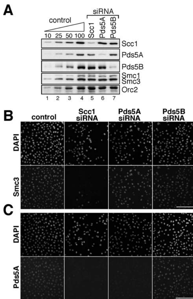
Fig. 3. Association of Pds5A with chromatin requires functional cohesin in HeLa cells. (A) HeLa cells were transfected with siRNAs specific to the cohesin subunit Scc1, Pds5A or Pds5B or mock-transfected with buffer as control. To estimate the extent of depletion, aliquots of siRNA-treated cell extracts were analyzed by immunoblotting (lanes 5-7) alongside increasing amounts of a control cell extract (expressed as percentage, lanes 1-4). The levels of Orc2 were analyzed as a loading control. (B,C) HeLa cells transfected as in A were pre-extracted with detergent before fixation and stained with DAPI and anti-Smc3 (B) or anti-Pds5A (C). All images were acquired over the same exposure time. Bar, 50 \mu m.
