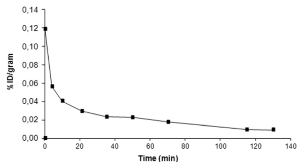
Fig. 4 TACs for [ ^{18}\text{F} ]-tetrafluoroborate in blood. TACs for [ ^{18}\text{F} ]-tetrafluoroborate expressed as percentage of the injected dose (ID) per gram of blood. Curves correspond to a single animal
