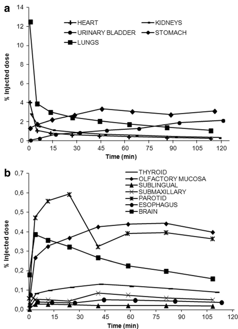
Fig. 3 TACs for [ ^{18}\text{F} ]-tetrafluoroborate in organs. TACs for [ ^{18}\text{F} ]-tetrafluoroborate in the most prominent organs: lung, heart, kidney, stomach and urinary bladder ( a ) and thyroid, olfactory mucosa, esophagus, brain and salivary glands (parotid, sublingual, submandibular) ( b ). Plots a and b have different ranges of radioactivity concentrations. Curves correspond to a single animal. TACs from the other monkey showed a similar pattern
