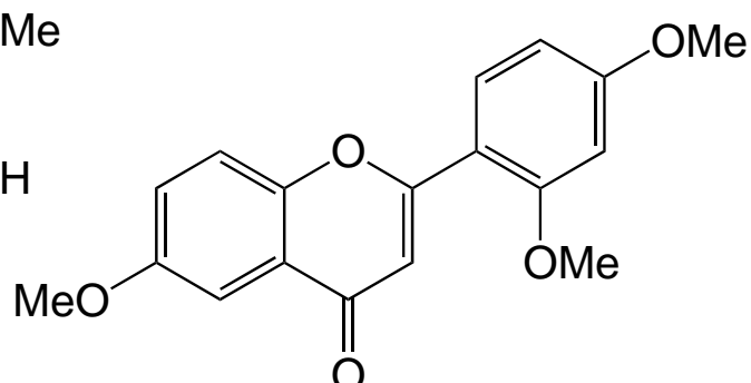
Trimethoxyflavone
