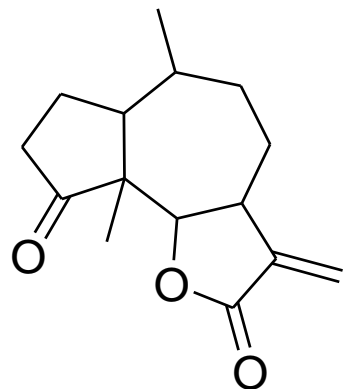
Damsin
