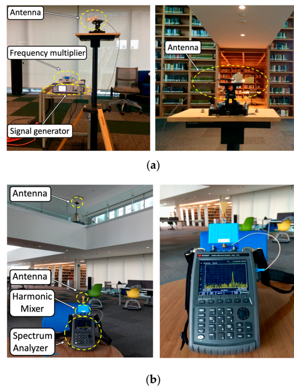
Figure 7. Measurement setup at 60 GHz frequency on the first and second floors of the library: (a) transmitter and (b) receiver.
