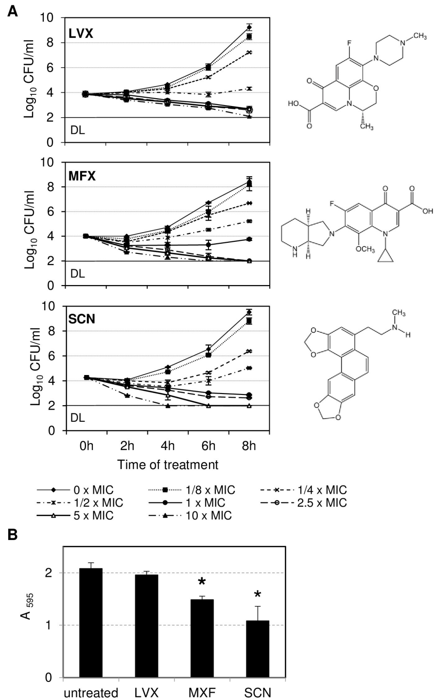
Fig 1. Bactericidal activity of drugs against strain S. pneumoniae R6. (A) Planktonic bacteria killing-curves in the absence or presence of the indicated drugs, which chemical structures are showed on the right. DL, detection limit (B) Inhibition of 6h-biofilm treated with 5 × MIC for 24 h, quantified by crystal violet staining. The results are the mean ± SD of two (A) and three (B) independent experiments. *, P < 0.05 versus untreated.
