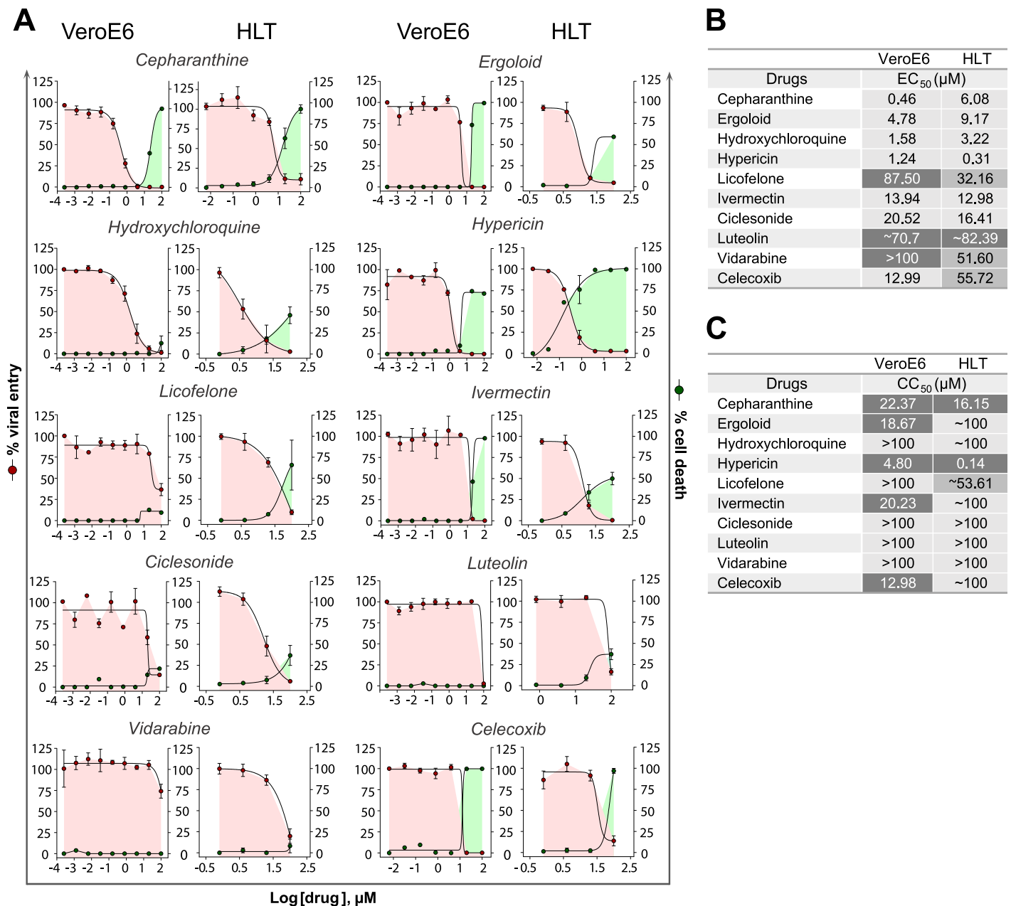
Fig 3. Antiviral assays with concordant results between models. (A). Percentage of viral entry in VeroE6 and HLT cells exposed to VSV ΔG (Luc)-Spike in the presence of cepharanthine, ergoloid, hydroxychloroquine, hypericin, licofelone, ivermectin, ciclesonide, luteolin, vidarabine and celecoxib. Drugs were used at concentrations ranging from 100 μM to 0.256 nM, in VeroE6, and to 0.8 μM in lung cells. Non-linear fit model with variable response curve from at least three independent experiments in replicates is shown (red lines). Cytotoxic effect on VeroE6 cells and HLT exposed to drug concentrations in the absence of virus is also shown (green lines). (B). EC 50 values of each drug in VeroE6 and HLT cells. (C). CC 50 values of each drug are shown for VeroE6 and for HLT cells.
