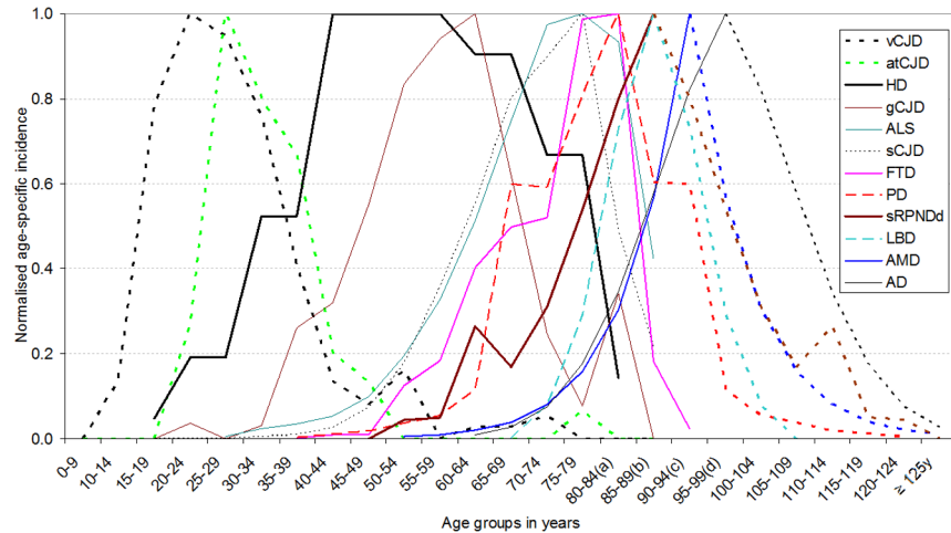
Fig 4. Reported and hypothesised (symmetrically replicated, dotted line) normalised incidence of sCJD, ALS, PD, LBD, AD, sRPNDd and AMD, assuming protracted population survival until 125 years for a substantial proportion of elderly. (a) 80–84 years is equivalent to 80 years and over for HD. (b) 85–89 years is equivalent to 85 years and over for sCJD, ALS. Abbreviations: Creutzfeldt-Jakob disease (CJD); accidentally transmitted CJD (atCJD), amyotrophic lateral sclerosis (ALS), motor neurone disease (MND), fronto-temporal dementia (FTD), Parkinson's disease (PD), Lewy body disease (LBD), age-related macular degeneration (AMD), Alzheimer's disease (AD), sporadic rapid-progressive neurodegenerative dementia (sRPNDd).
