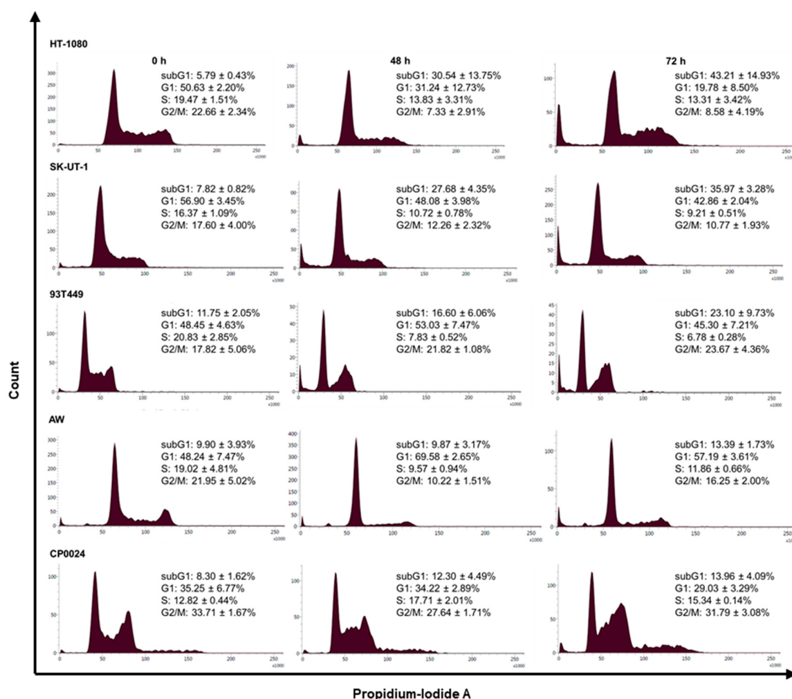
Figure S1. Inhibition of CBP/ \beta -catenin interaction promotes cell death in STS cells. Cells were treated with PRI-724 (10 \mu M), fixed with ethanol, stained with propidium iodide, and DNA content was determined by flow cytometry. Histograms of PRI-724-treated cells for 0, 48 and 72 h are shown. The fluorescence values (count) used to calculate the peaks corresponding to the sub-G1, G1 and the G2/S/M phase are indicated on each histogram.
