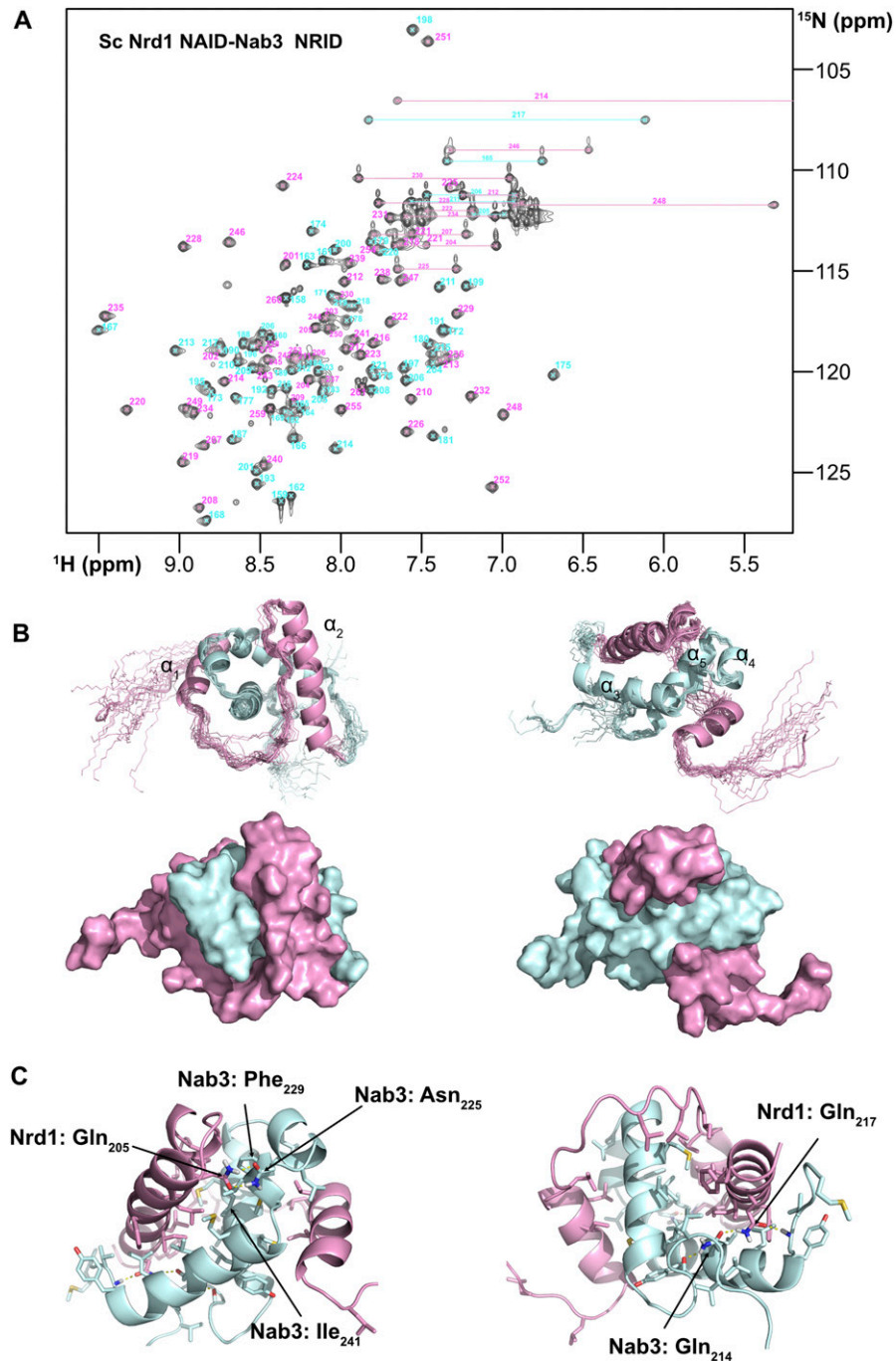
Figure 3. Nuclear magnetic resonance structure of the Nrd1-Nab3 chimera. (A) ^1\text{H} - ^{15}\text{N} HSQC spectrum of the Nrd1 158-222 -Nab3 202-261 chimera recorded at 800 MHz and 25°C. Cross-peaks assignments have been labelled according to the amino acid sequences of Nrd1 (in pink) and Nab3 (in cyan) fragments that compose the chimera. The horizontal lines mark the two cross-peaks of amide NH 2 moieties in side chains of Gln and Asn residues. (B) Superposition of the 20 structural models calculated by nuclear magnetic resonance (statistics in Table S1) (upper panels) (PDB code: 7PRD). Two different orientations are shown. The Nrd1 in the chimera is colored in light pink and the Nab3 part in light cyan. Regular secondary structure elements are named consecutively ( \alpha -helices \alpha_1 to \alpha_5 ). Surface representations of the structure in the two selected orientations and with the same color code are shown below. (C) Structural details of the interaction between Nrd1 and Nab3 parts of the chimera. Only side chains of residues involved in heterodimeric contacts are shown. The interface is mainly formed by hydrophobic residues with the exception of Nrd1 Gln 205 and Gln 217 with Nab3 Gln 214 and Asn 225 that participate in two hydrogen bond networks (yellow dashed lines) that are buried inside the structure. The Nab3 Phe 229 -Ile 241 contact, present in the free form (Fig 1E), is maintained in the Nrd1-Nab3 chimera. (B) Residues have been numbered according to the Nrd1 and Nab3 sequences and colored as in panel (B).
