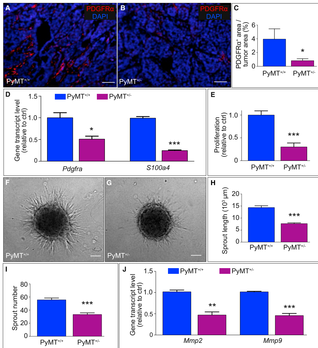
Figure 3. Effect of PHD2 Haploinsufficiency on CAF Activation and Invasion
