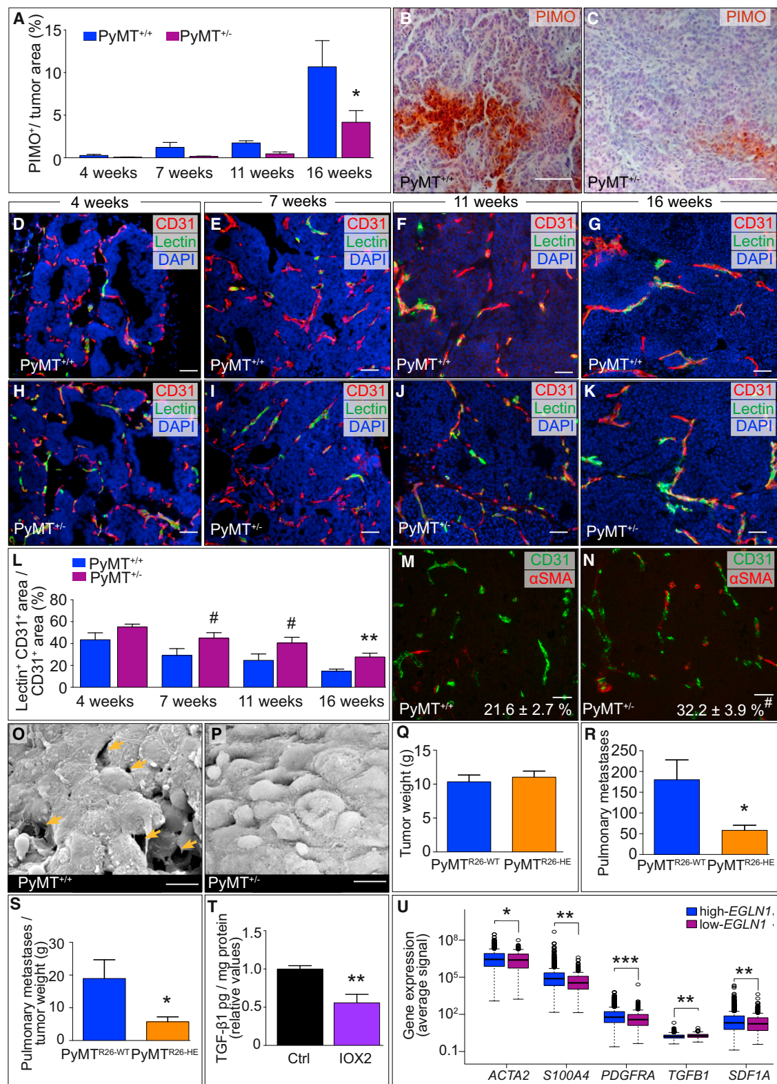
Figure 7. Effect of PHD2 Haploinsufficiency on Tumor Vessels and Translational Studies
