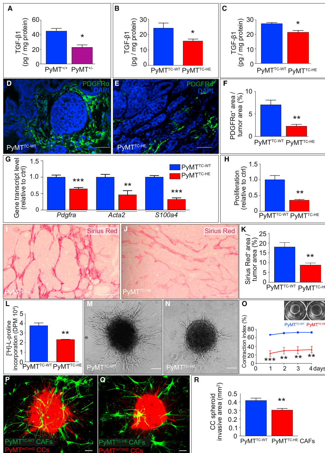
Figure 5. Effect of Cancer Cell PHD2 Haploinsufficiency on Paracrine TGF-β1 Crosstalk between Cancer Cells and CAFs
