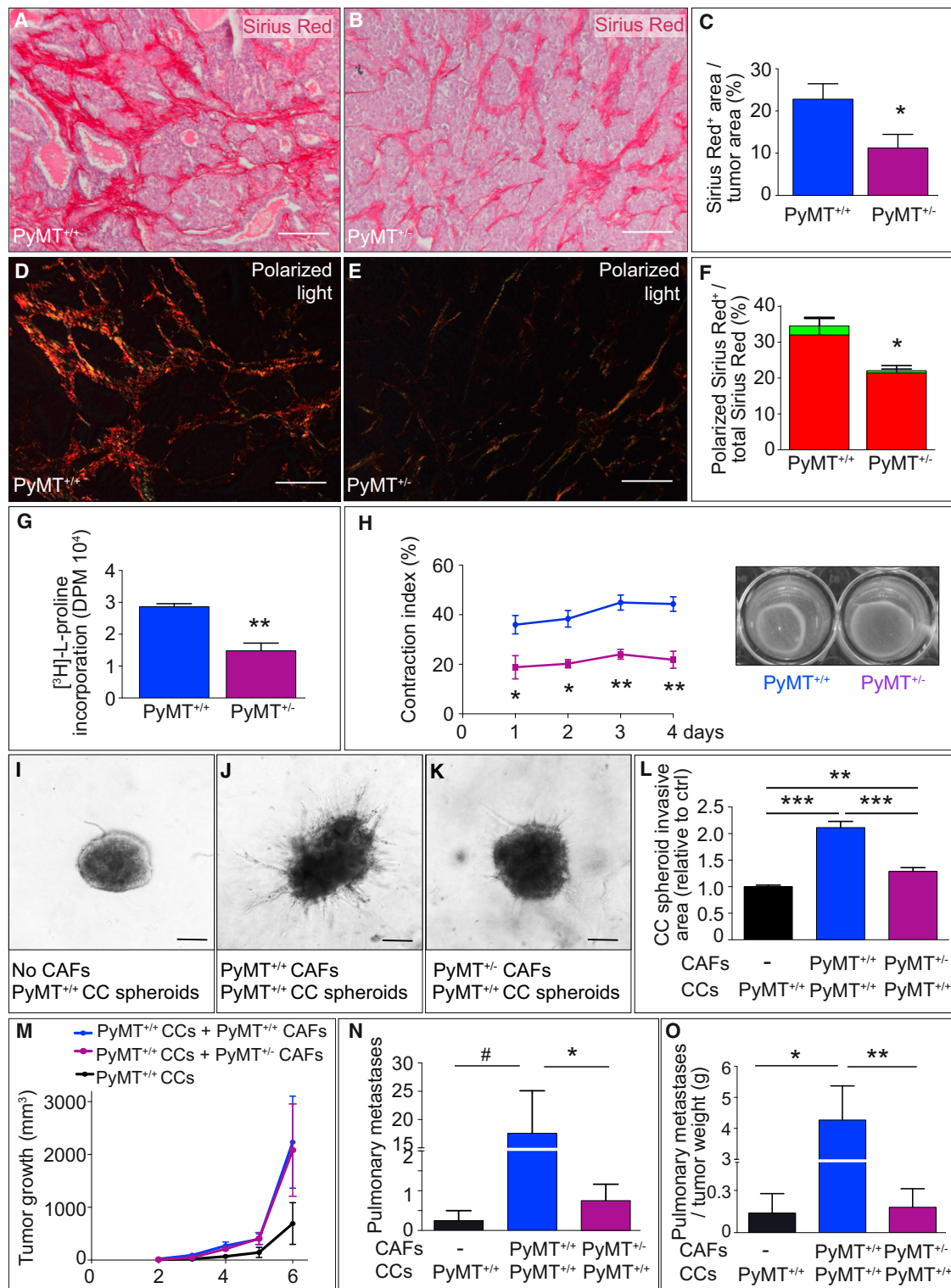
Figure 4. Effect of PHD2 Haploinsufficiency on Matrix Production and Remodeling by CAFs
