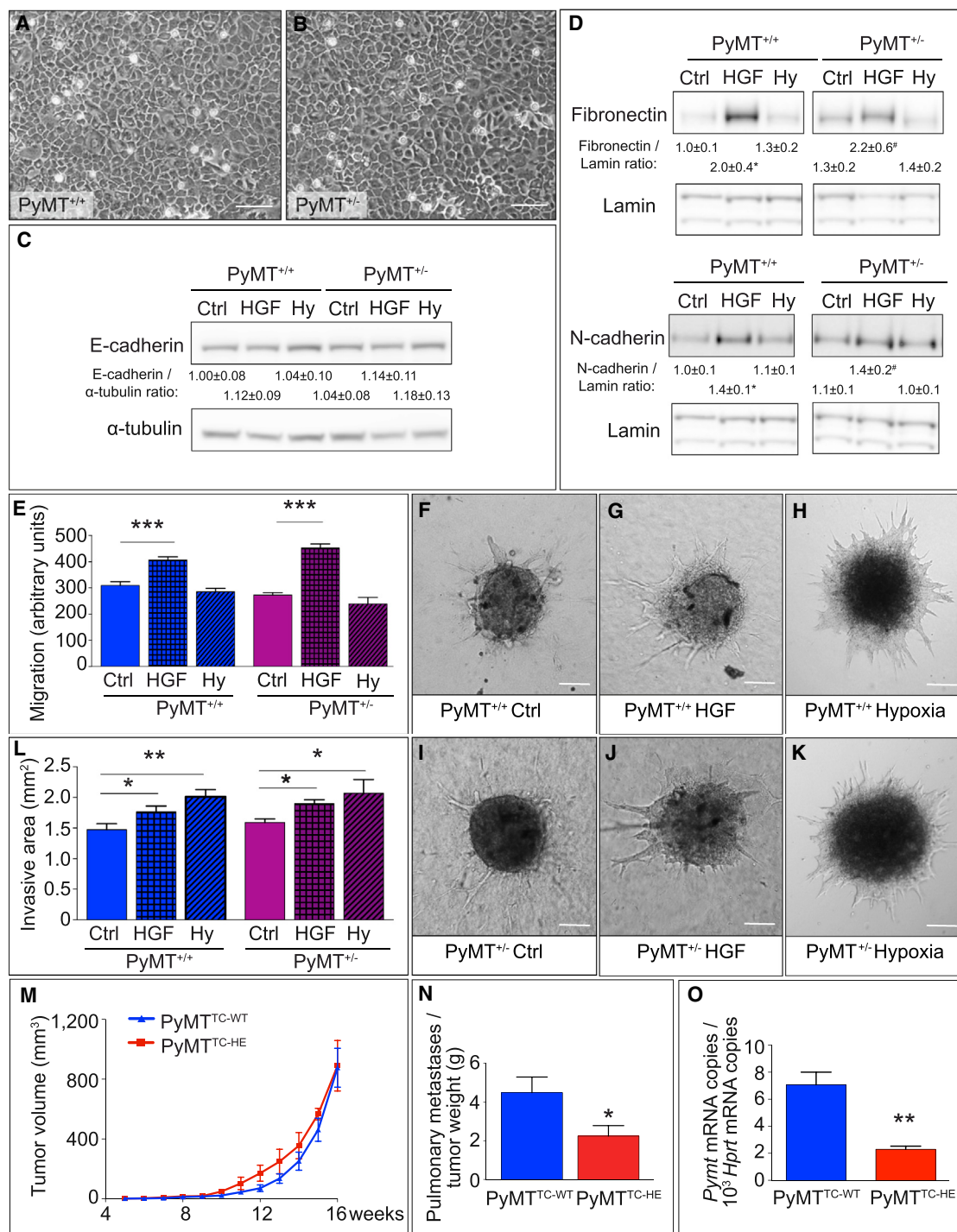
Figure 2. Effect of PHD2 Haploinsufficiency on Cancer-Cell-Intrinsic Invasive Properties
