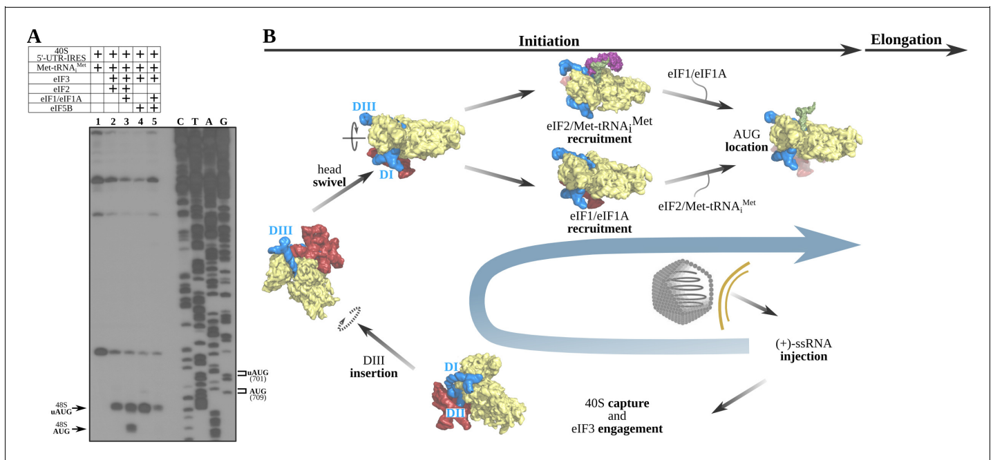
Figure 6. The 5'-UTR-IRES requires TC, eIF1 or eIF1A to assemble a functional initiation complex via an uAUG intermediate. (A) Toe-print analysis of 48S initiation complexes assembled on 5'-UTR-IRES in an in vitro reconstituted system. eIF2 delivers Met-tRNA Met to the uAUG (lane 2) and requires the presence of eIF1 or eIF1A to transition to the bona fide AUG codon of ORF1 (lane 3). Under some conditions, eIF5B can substitute for eIF2 in Met-tRNA Met delivery (Terenin et al., 2008). In the absence of eIF1 or eIF1A, a robust toe-print signal is detected in the presence of eIF5B (lane 4), however, Met-tRNA Met is delivered to the uAUG, and thus eIF5B is unable to find the annotated AUG even in the presence of eIF1 or eIF1A (lane 5). (B) A model for 5'-UTR-IRES-mediated translation initiation. From the bottom right: injection of the genomic (+)-ssRNA of the CrPV into the cytosol allows the 5'-UTR-IRES to capture free 40S and eIF3, which is recruited to the complex with an initial canonical conformation of the 40S head without tilt or swivel. Insertion of 5'-UTR-IRES DIII in the vicinity of the E-site and a swiveling movement of the 40S head induces a 'locked' conformation of the complex, with the uAUG at 701 in the vicinity of the P-site. Delivery of Met-tRNA Met and location of ORF1 AUG is achieved by the concerted action of eIF2, eIF1 and eIF1A. Large subunit recruitment mediated by eIF5B will allow transitioning into elongation. The online version of this article includes the following figure supplement(s) for figure 6:
