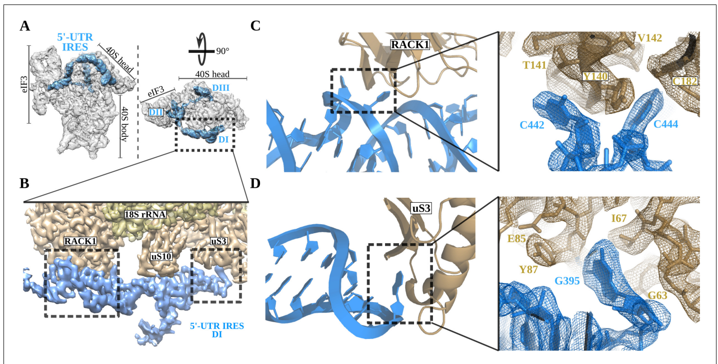
Figure 2. The 5'-UTR-IRES domain I engages ribosomal proteins RACK1 and uS3. (A) Overview of the 40S-5'-UTR-IRES-eIF3 map, with 40S and eIF3 depicted gray and 5'-UTR-IRES in blue. (B) Detailed view of the cryo-EM density of the 40S-5'-UTR-IRES-eIF3 map centered around 5'-UTR-IRES domain I (DI). Ribosomal proteins are colored brown, 18S rRNA yellow and 5'-UTR-IRES blue. Contacts between 5'-UTR-IRES domain I and ribosomal proteins RACK1 (C) and uS3 (D) could be defined thanks to well-resolved local cryo-EM densities.
