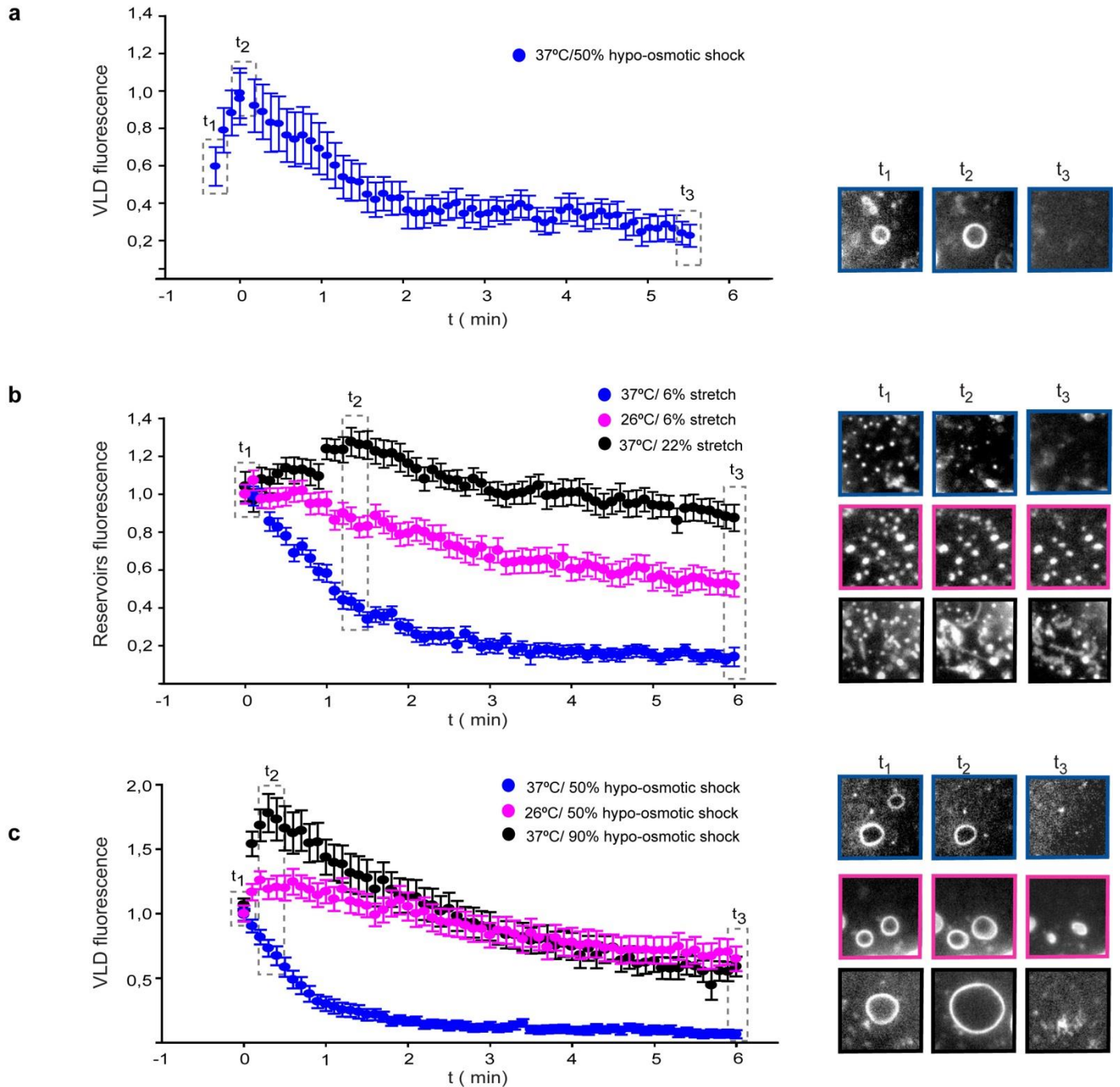
Supplementary Figure 3. Dynamic formation and resorption of membrane structures. a , Quantification of VLD fluorescence after re-application of iso-osmotic medium (1: maximum fluorescence, 0: background). n = 20 VLDs from 2 cells. Imaging was carried out using an inverted microscope (60x objective) which allowed to visualize the initial VLD formation period. b , Quantification of reservoir fluorescence after stretch release (1: initial fluorescence, 0: background). n = 100/80/30 reservoirs from 10/3/3 cells. Imaging was carried out using an upright microscope (60x objective). Both decreasing temperature (pink symbols) and increasing stretch magnitude (black symbols) slowed the process of reservoir formation. Images to the right show corresponding examples of membrane structures at the times indicated in the graph. c , Quantification of VLD fluorescence after re-application of iso-osmotic medium (1: initial fluorescence, 0: background). n = 100/50/60 VLDs from 10/5/4 cells. Imaging was carried out using an upright microscope (60x objective). Both decreasing temperature (pink symbols) and increasing the magnitude of the hypo-osmotic shock (black symbols) slowed the process of VLD formation. Images to the right show corresponding examples of membrane structures at the times indicated in the graph. All insets have a size of 10 \times 10 \mu\text{m} .
