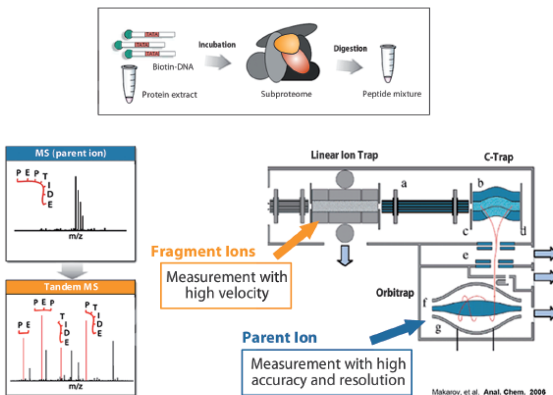
Protein identification of a complex mixture in the Thermo LTQ Orbitrap XL mass spectrometer
