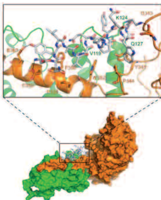
Docking and molecular dynamic simulations of binding between calcineurin and the NFAT-derived LxVP peptide. LxVP (sticks) is positioned parallel to the \beta -subunit-binding helix of CnA (orange) and forms additional contacts with residues in CnB (green).
