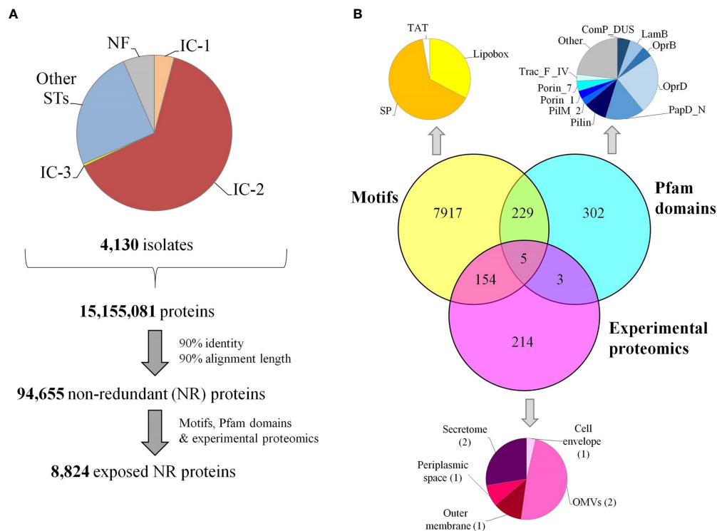
FIGURE 2 | Pan-proteome data management and selection of exposed proteins. (A) Flowchart indicating pan-proteome data collection, redundancy reduction and exposed protein selection. Genomic representation of international clones is shown. (B) Identification of exposed proteins by three approaches. OMVs, outer membrane vesicles; SP, signal peptides transported by the Sec translocon; TAT, signal peptides transported by the Tat translocon.
