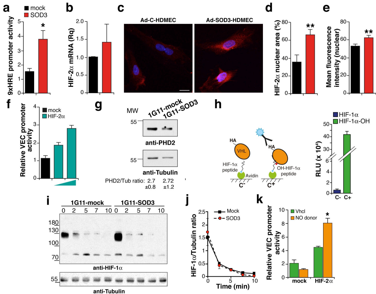
Supplementary Figure 9. SOD3 and NO regulate HIF-2α stability and transcriptional activity. (a) Relative activity of a 9xHRE synthetic promoter in mock- or SOD3-transfected 1G11 cells ( n = 3 ). (b) Basal HIF-2α mRNA levels in mock- or SOD3-transfected 1G11 cells ( n = 4 ). (c) Representative images of HIF-2α staining in Ad-C- and Ad-SOD3-infected HDMEC cells ( n \geq 250 cells/condition). (d, e) Percentage of nuclear area and mean fluorescence intensity in images as in c. (f) Relative VEC promoter activity in 3T3 cells transfected with increasing quantities of HIF-2α plasmid (green bars). An empty plasmid was used as control (black bar; n = 3 ). (g) Immunoblot analysis of lysates from 1G11-mock and -SOD3 cells with anti-PHD2 and -tubulin (loading control) antibodies; the ratio (mean \pm SEM) is indicated at bottom ( n = 3 ). (h) Diagram of the ELISA designed to analyze specificity of recombinant-produced, HA-tagged VHL protein (left). The graph shows the result of a representative ELISA (right). HA-VHL binding to the hydroxylated HIF-1α peptide is >40 -fold higher than the non-hydroxylated peptide. RLU, relative luciferase units. (i) Representative immunoblot of HIF-1α levels after re-oxygenation of cycloheximide-treated 1G11-mock and -SOD3 cells cultured in hypoxia; tubulin was used as loading control. (j) HIF-1α/tubulin ratio obtained by densitometric quantification of immunoblots as in i ( n = 3 ). No significant differences were observed between cell lines; two-way ANOVA with Bonferroni post-hoc correction. (k) 3T3 cells were cotransfected with HIF-2α (or empty vector as control) and the VEC promoter, and incubated with DETA-NONOate (NO donor) or Vhcl; the relative luciferase activity driven by the VEC promoter was then measured ( n = 5 ). (a, b, d, e-h, j, k) Data shown as mean \pm SEM of triplicates; * p < 0.05 , ** p < 0.01 , two-tailed Student's t-test. Bar, 20 \mu m.
