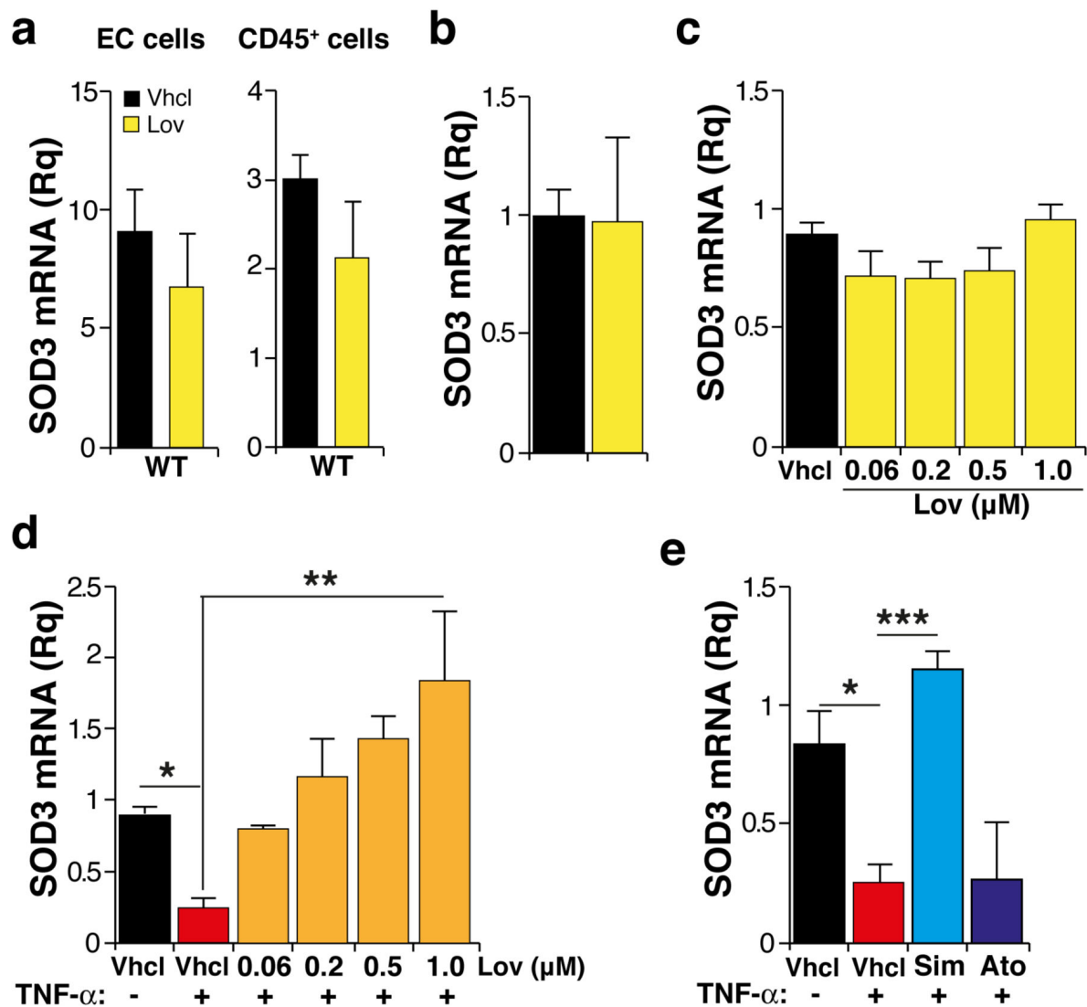
Supplementary Figure 3. Lov induces SOD3 through an indirect mechanism. (a) Relative SOD3 mRNA levels in endothelial cells isolated from lung and in leukocytes isolated from spleen of tumor-free mice treated with Vhcl or Lov as indicated. Data are mean \pm SEM of triplicates ( n = 4 ). Values were not statistically different; two-tailed Student's t -test. (b) Effect of Lov ( 1 \mu\text{M} ) on SOD3 mRNA levels in 1G11 cells. Differences were not significant; two-tailed Student's t -test. (c) Effect of different Lov doses on SOD3 mRNA levels in 3T3 cells. Values were not statistically different; one-way ANOVA with Dunnet's post-hoc test, using Vhcl as reference. (d) 3T3 cells were incubated for 48 h with TNF- \alpha and the indicated doses of Lov or the corresponding Vhcl (see Methods); SOD3 mRNA levels were determined by RT-qPCR. (e) 3T3 cells were incubated (48 h) with TNF- \alpha and either simvastatin (Sim) or atorvastatin (Ato), or their corresponding Vhcl. For b-e , data are mean SEM of triplicates ( n = 3 ). * p < 0.05 , ** p < 0.01 , one-way ANOVA with Tukey's post-hoc test.
