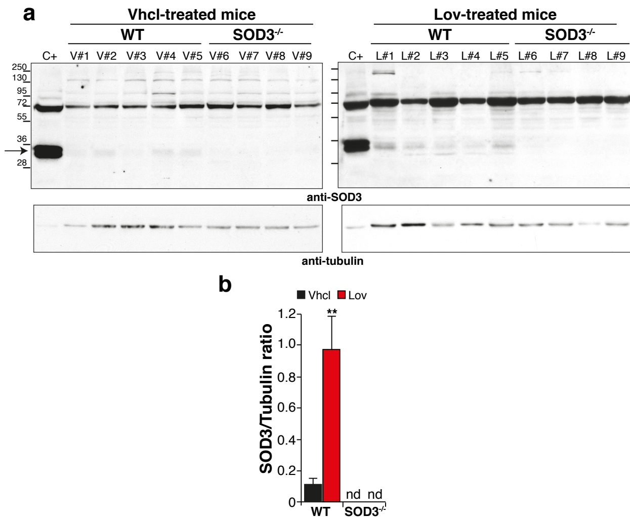
Supplementary Figure 2. Lovastatin treatment induces SOD3 upregulation in LLC tumors. (a) Immunoblot analysis of extracts of representative LLC tumors grown in Vhcl- or Lov-treated WT or SOD3 -/- mice, using anti-SOD3 (top) or anti-tubulin antibodies (bottom; loading control). C+ is a lung tissue extract used as positive control for SOD3. (b) The intensity of SOD3- and tubulin-specific bands was measured by densitometry, and the ratio calculated for individual tumor samples. The graph shows mean ± SEM of the SOD3/tubulin ratio in Vhcl- and Lov-treated mice ( n = 10/\text{group} ); nd, not detected. ** p < 0.01 , two-tailed Student's t -test.
