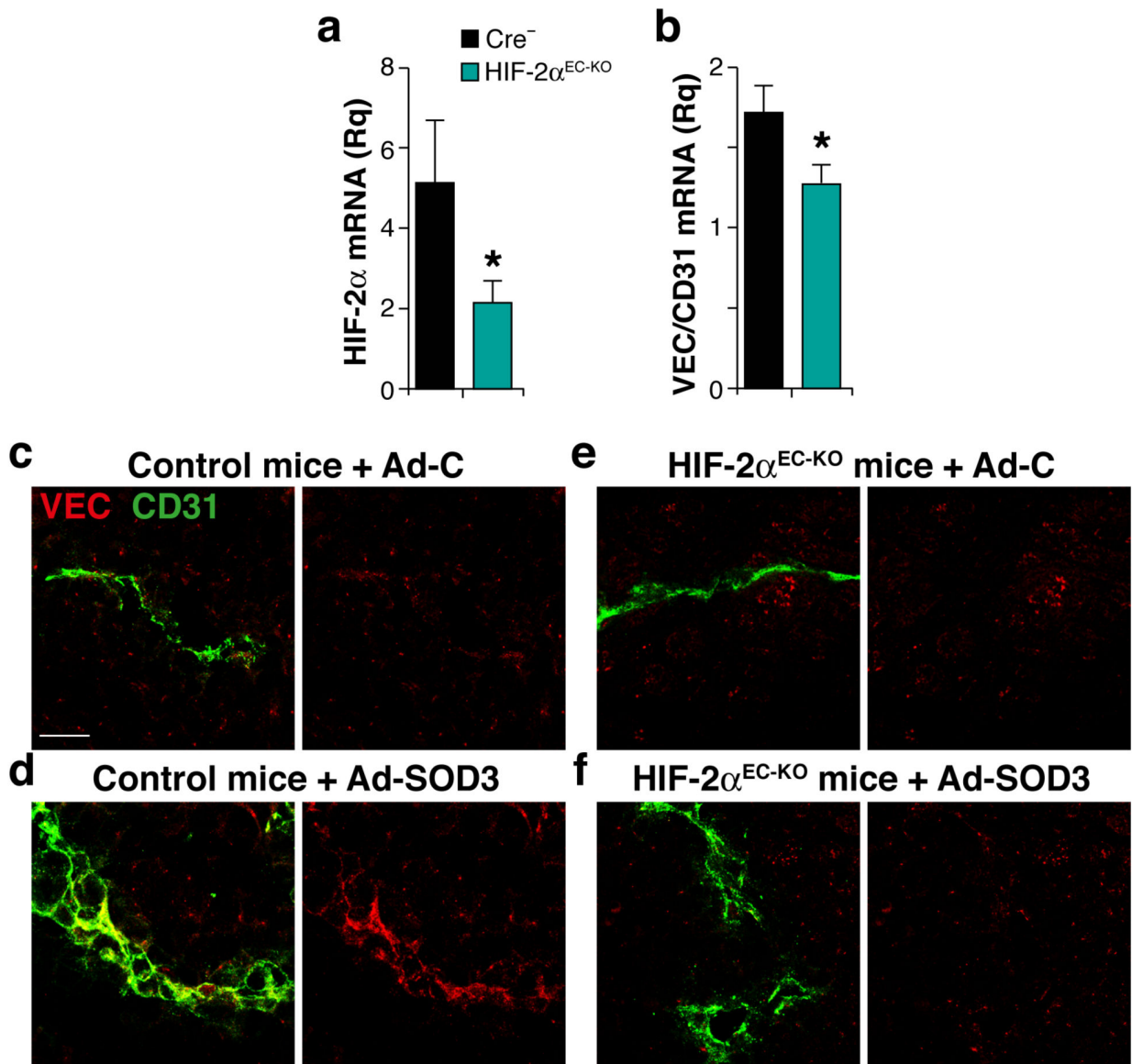
Supplementary Figure 10. HIF-2α mediates SOD3-induced VEC transcription in vivo. (a, b) Relative HIF-2α and VEC mRNA levels in EC isolated from tumors grafted in control (Cre - ) and HIF-2α EC-KO mice. Data shown as mean ± SEM of triplicates from 4 mice/genotype. * p < 0.05, two-tailed Student's t -test. (c-f) Immunofluorescence images of VEC (red) and CD31 (green) staining in tumors from Ad-C- and Ad-mSOD3-treated control (Cre - ) and HIF-2α EC-KO mice. Bar, 20 μm.
