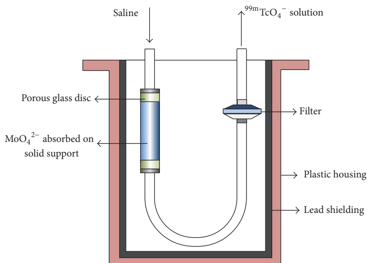
FIGURE 4: General scheme of a ^{99}\text{Mo}/^{99\text{m}}\text{Tc} generator.
