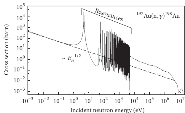
FIGURE 8: Excitation function for the neutron capture reaction ^{197}\text{Au}(n,\gamma)^{198}\text{Au} . The oscillations of the reaction cross section in the energy range between 5 and 5000 eV are referred to as resonances (data from JEFF 3.1.1 (OECD-NEA 2009)).
