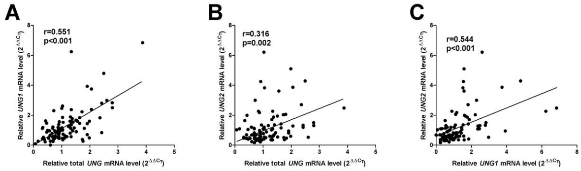
Figure S1. A) Correlation analysis between total UNG mRNA expression and UNG1 mRNA expression. B) Correlation analysis between total UNG mRNA expression and UNG2 mRNA expression. C) Correlation analysis between UNG1 mRNA and UNG2 mRNA expression. Spearman's test was used to assess the significance of the correlations.
