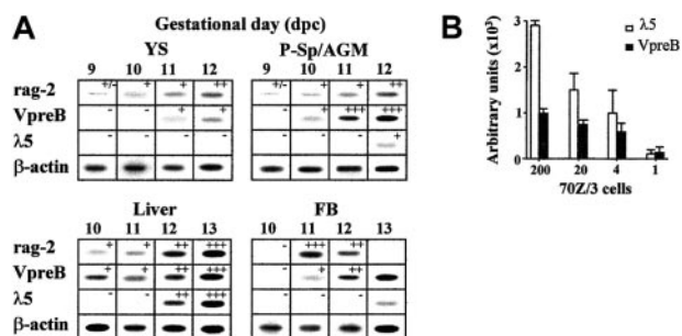
Figure 1. Expression of lymphoid lineage-specific genes in midgestation (9-13 dpc) mouse embryos. (A) Gene transcript levels of rag-2 , VpreB , λ5 , and β-actin in sequential samples of embryo lymphohematopoietic progenitor-containing areas (YS, P-Sp/AGM, liver, and blood), as detected by semiquantitative RT-PCR. After hybridization and densitometric quantification, the means of the relative message levels obtained for rag-2 , VpreB , and λ5 were referred to those calculated in simultaneous 13-dpc liver PCR amplifications (as a maximum; n = 6-10 independent samples per organ per gestational day). These results are expressed by the +/– symbols in the figure, which represent –, < 1%; +/–, 1%-10%; +, 10%-40%; ++, 41%-70%; +++, 71%-100%. (B) Sensitivity threshold of λ5 - and VpreB -specific RT-PCRs calculated in a titration of the 70Z/3 pre-B-cell line up to the single-cell level. Densitometric quantification of the specific signals obtained in 3 independent experiments; means \pm SD are shown.
