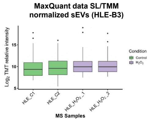
Supplementary Fig. 1. Box plots for the TMT data before and after SL/TMM normalization.
