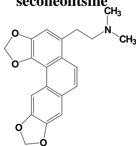
#16: N-methyl-seconeolitsine
