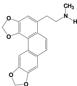
#17: Seconeolitsine
