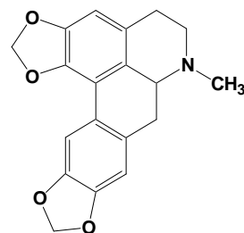
#14: Neolitsine
