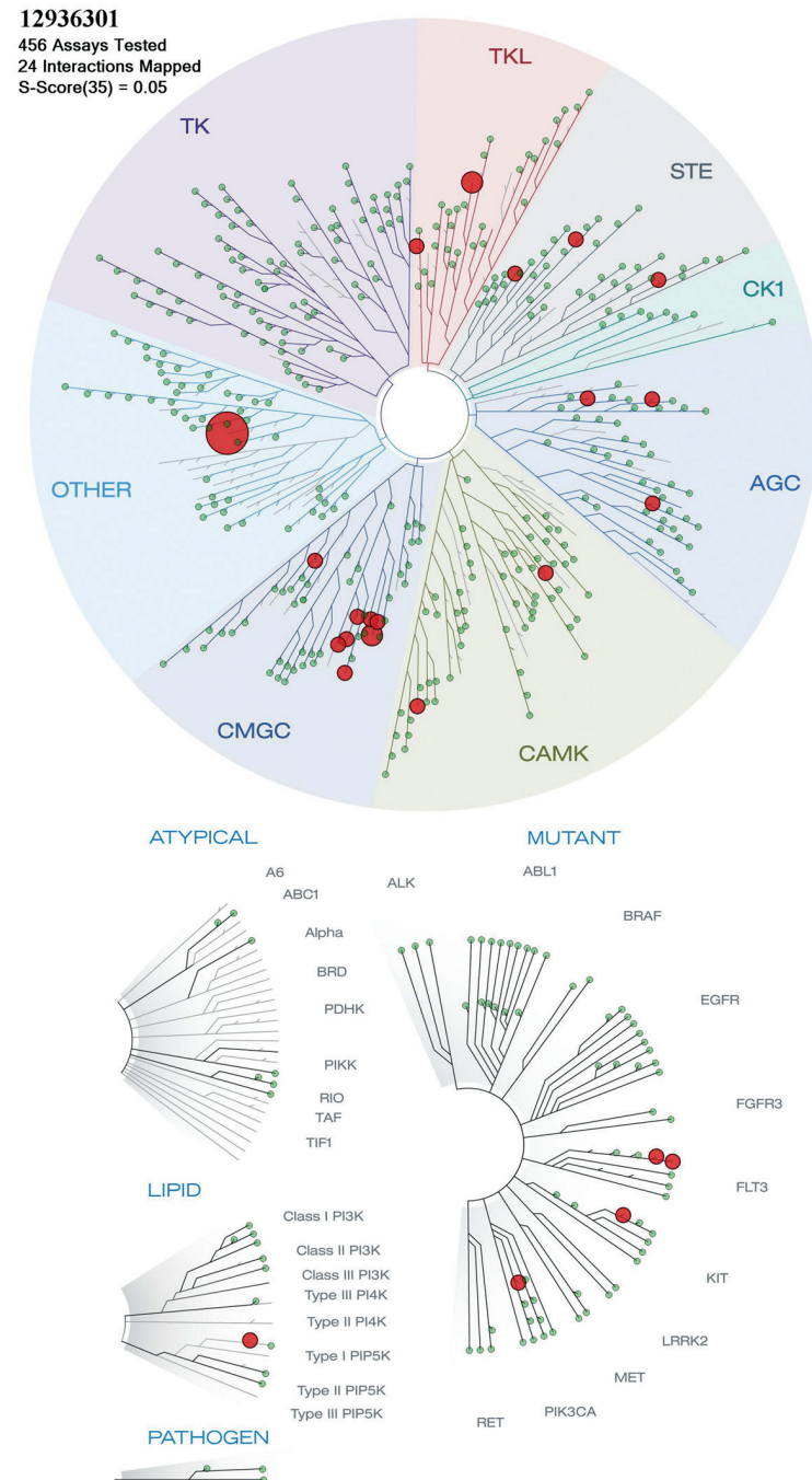
Figure A selected CDK8 inhibitor tested in a 456 kinase panel (KINOMEScan). The selectivity score of the compound S(35) is 0.05. A representation of the selectivity profile of S(35) for 38 small molecule kinase inhibitors indicates the selectivity of our compound. Kinases that are found to bind are marked with red circles - whereas larger circles indicate higher binding affinity. Only 1
