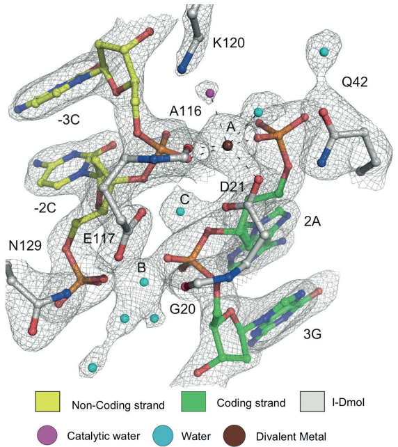
Figure 2 Detailed view of the I-Dmol active site, superimposed with the 2F_o - F_c electron density contoured at 1.2\sigma . Metal-ion coordination is shown as dashed lines. The different metal-binding sites are alphabetically labelled (site A, B and C) according to the order of cation entrance.
