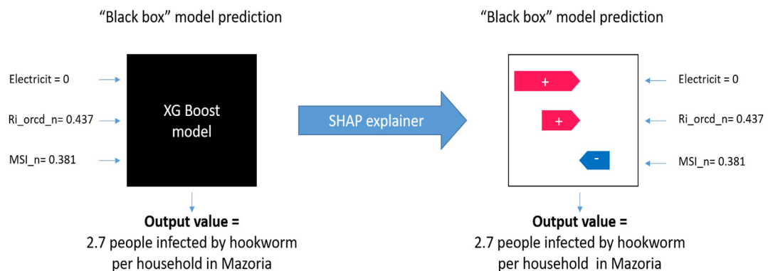
Fig. 3. Diagrammatic representation of SHAP. Figure adapted from Lundberg et al. (2020). From local explanations to global understanding with explainable AI for trees. Nature machine intelligence , 2(1), 56–67. The values and variables shown in this figure were taken from the force plot presented in Fig. 6.
