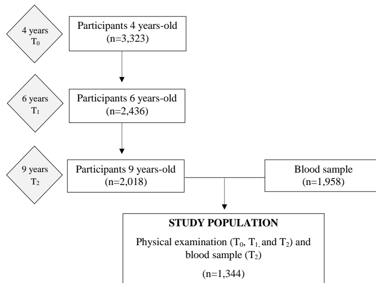
Figure S1. Flowchart of participants enrolment
