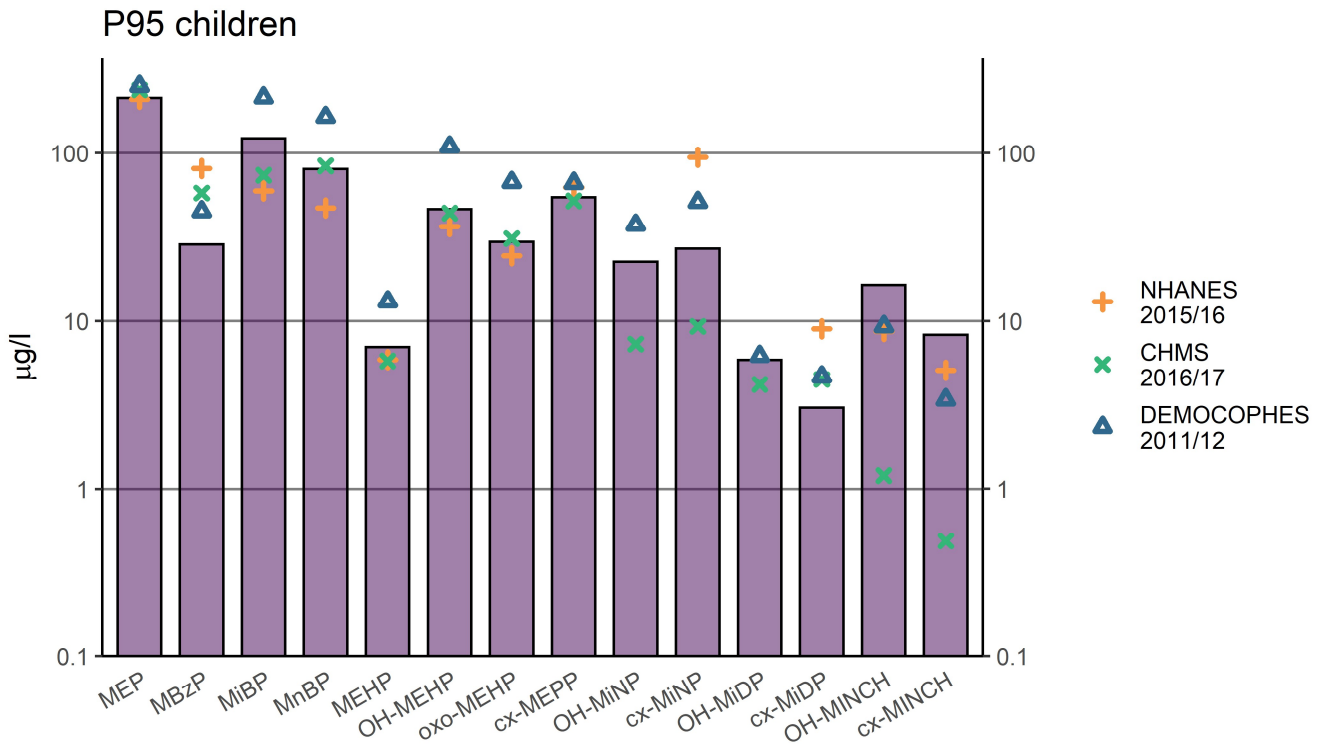
Supplementary Figure 1. P95 ( \mu\text{g/L} ) of children (6-11) from HBM4EU Aligned Studies (2014-2021) compared to P95 from the comparable age group in NHANES (2015-2016), CHMS (2016-2017) and DEMOCOPHES (mean of available country P95s, 2011-2012) by phthalate and DINCH metabolites.
