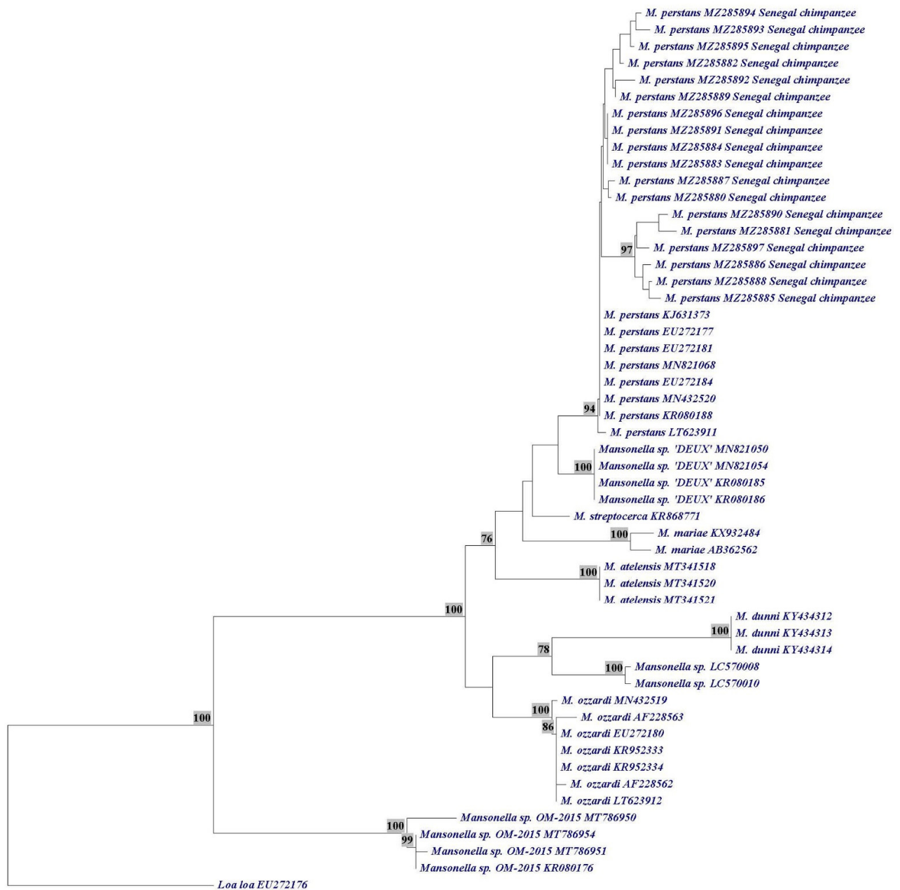
Figure S3. Mansonella spp. ITS1 phylogenetic tree. Phylogenetic relationships among Mansonella perstans sequences identified in free-living chimpanzees in the present study (labeled as Senegal Chimpanzee) and homologous sequences retrieved from GenBank (Sequence accession numbers are indicated). The analysis was conducted by the neighbor-joining method of the ITS1 of the rRNA gene using Treecon software [96] after ClustalW alignment of the sequences [97]. Bootstrap values (1000 replicates) lower than 75% are not displayed. Loa loa was used as outgroup to root the tree.
