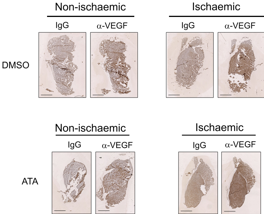
Figure S6. Experimentally-induced murine hind limb ischaemia is accompanied by upregulation of VEGF expression. Immunohistochemistry staining of VEGF in histological sections of non-ischaeamic (sham-operated) or ischaemic tibialis muscle isolated from mice treated with vehicle (DMSO) or ATA (5 mg/kg/day) for 10 days. A rabbit anti-VEGF ( \alpha -VEGF) polyclonal antibody (1.4 \mu g/ml, final concentration) was used to detect VEGF expression. Staining using rabbit IgG (IgG) at the same concentration was used as negative control. Scale bars, 1 mm.
