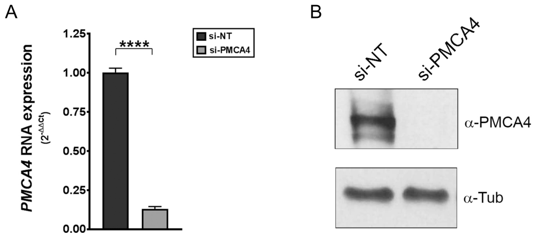
Figure S2. Small interfering RNA (siRNA) mediated knockdown of PMCA4 expression in endothelial cells. (A) PMCA4 RNA levels in HUVECs transfected with a non-targeting control siRNA (si-NT) or a siRNA specific for human PMCA4 (si- PMCA4 ) were determined by qRT-PCR. Histograms show data as mean \pm SE, n=9 , obtained from 3 independent experiments. Data were analysed for statistically significant differences by unpaired two-tailed Student t test. **** indicates statistically significant differences ( P \leq 0.001 ). (B) Analysis of PMCA4 protein expression in HUVECs transfected as in (A) using the anti- PMCA4 specific JA3 monoclonal antibody ( \alpha - PMCA4 ) or an anti-tubulin ( \alpha -Tub) antibody as a loading control. Western blot images are representative of 3 independent experiments.
