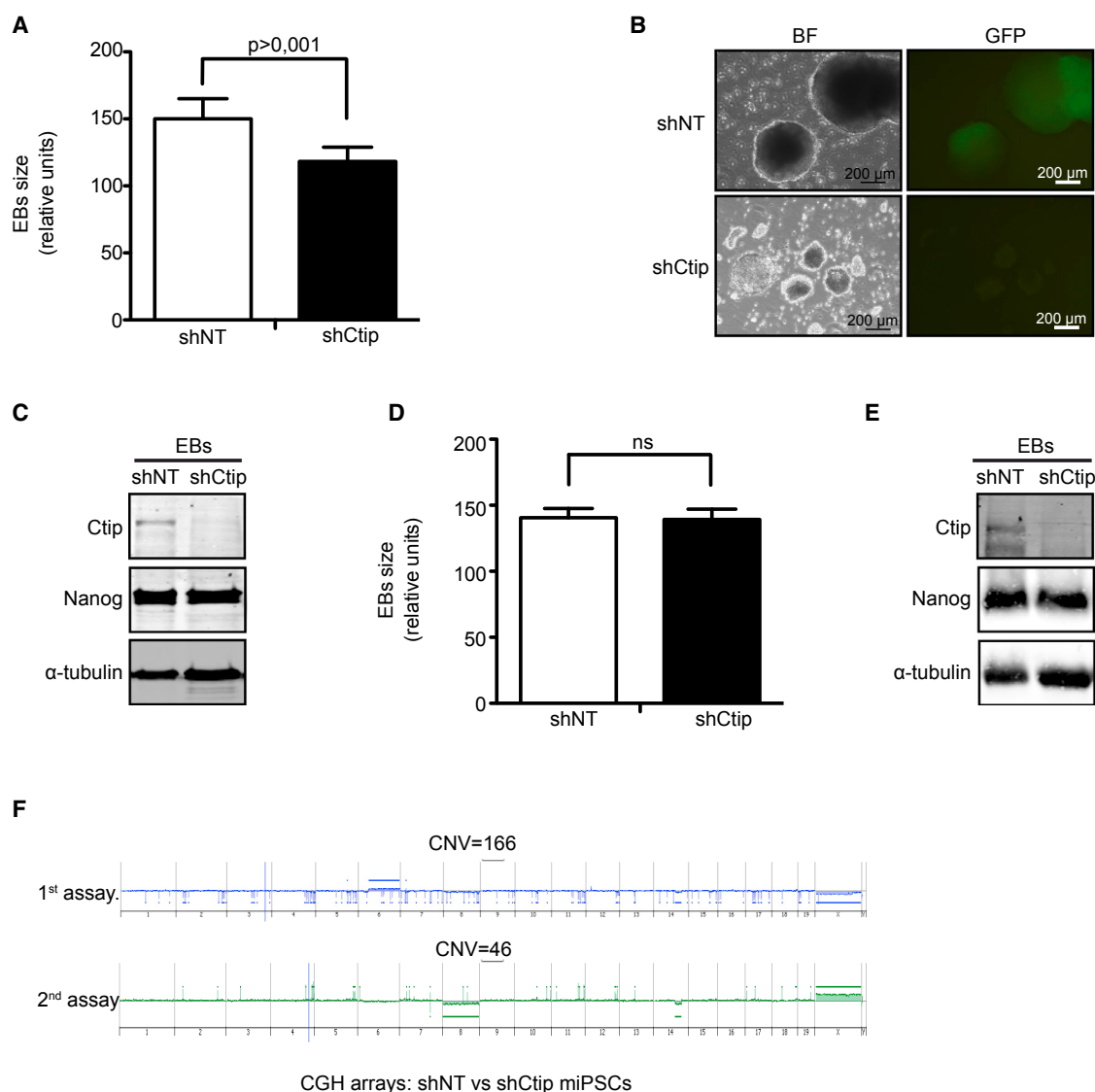
Figure 5. CtIP Is Essential for Differentiation and Genomic Stability Maintenance in iPSCs
