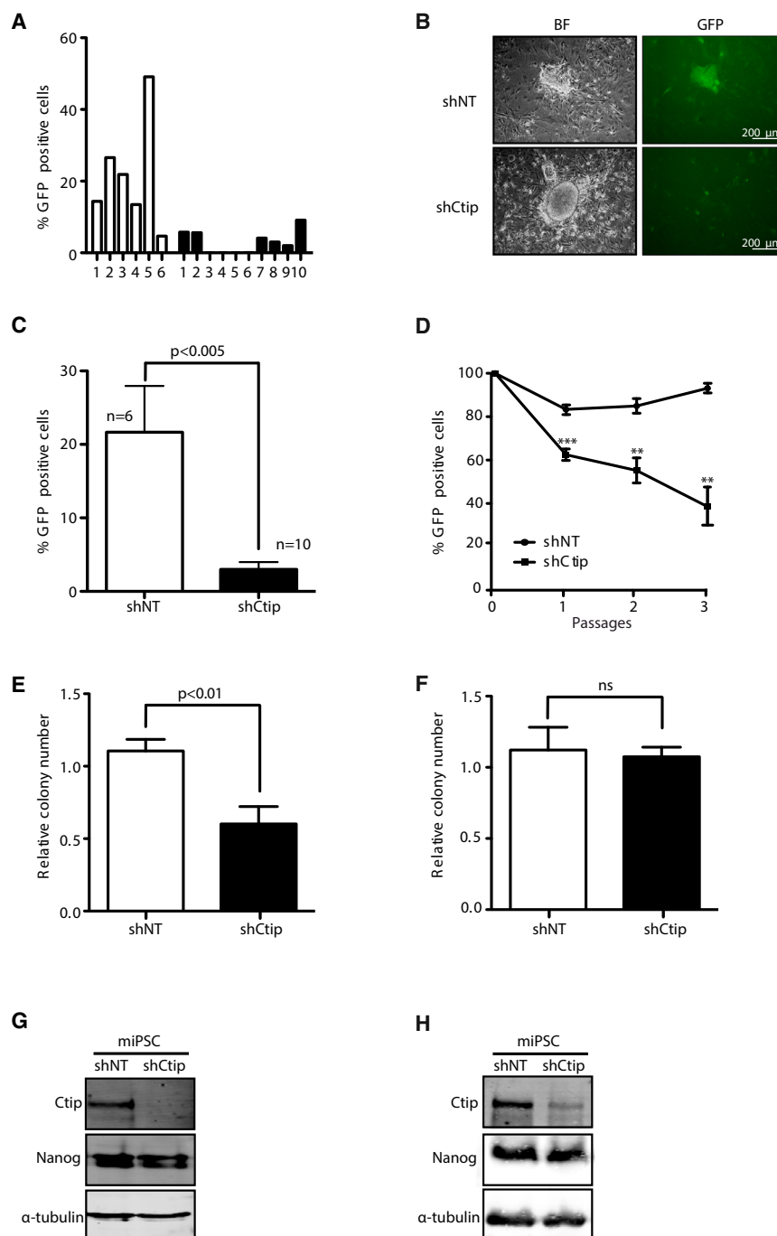
Figure 4. The Levels of CtIP During Reprogramming Affect iPSC Maintenance
