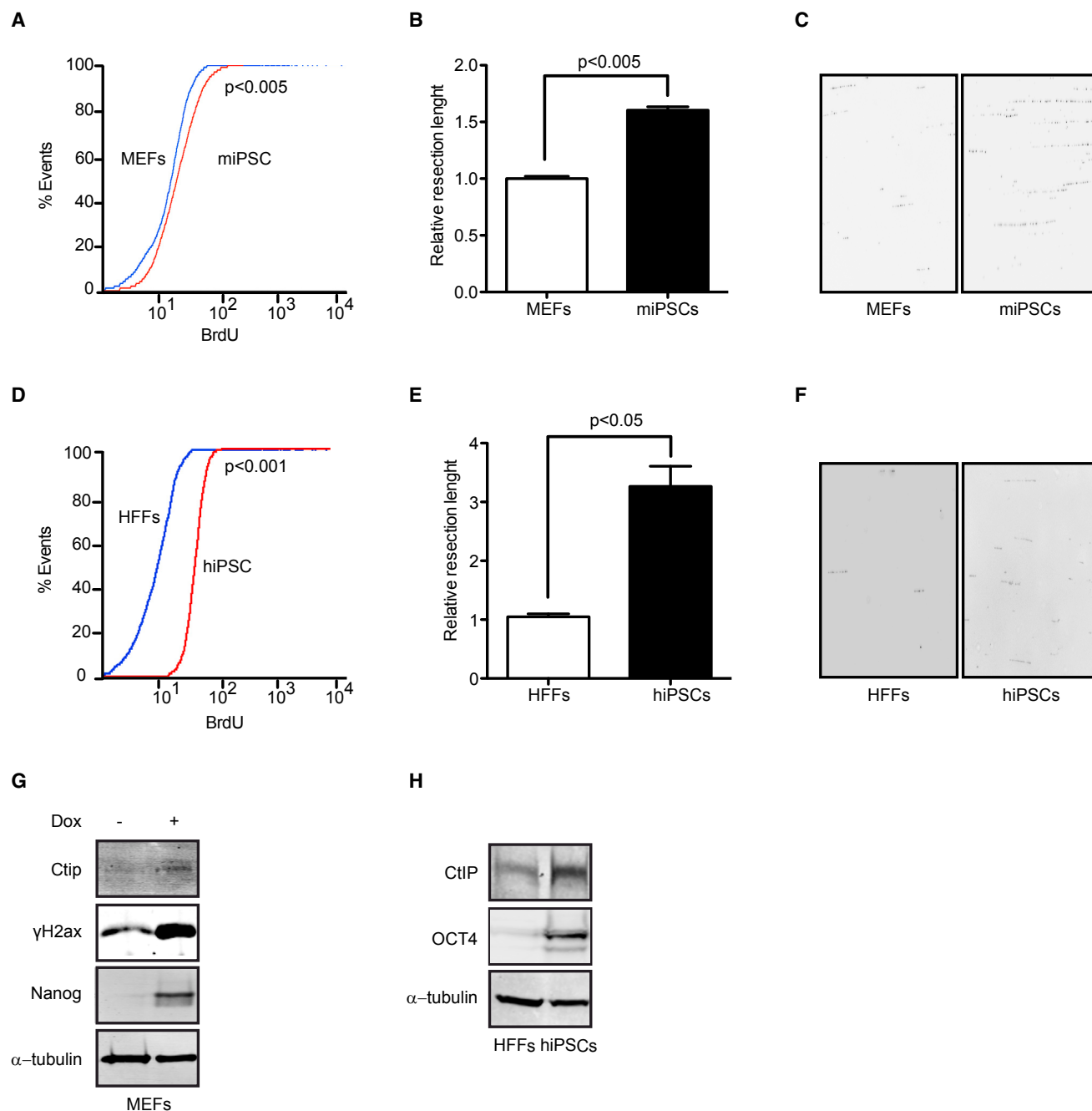
Figure 1. DNA End Resection Is an Essential Mechanism for Cell Reprogramming
