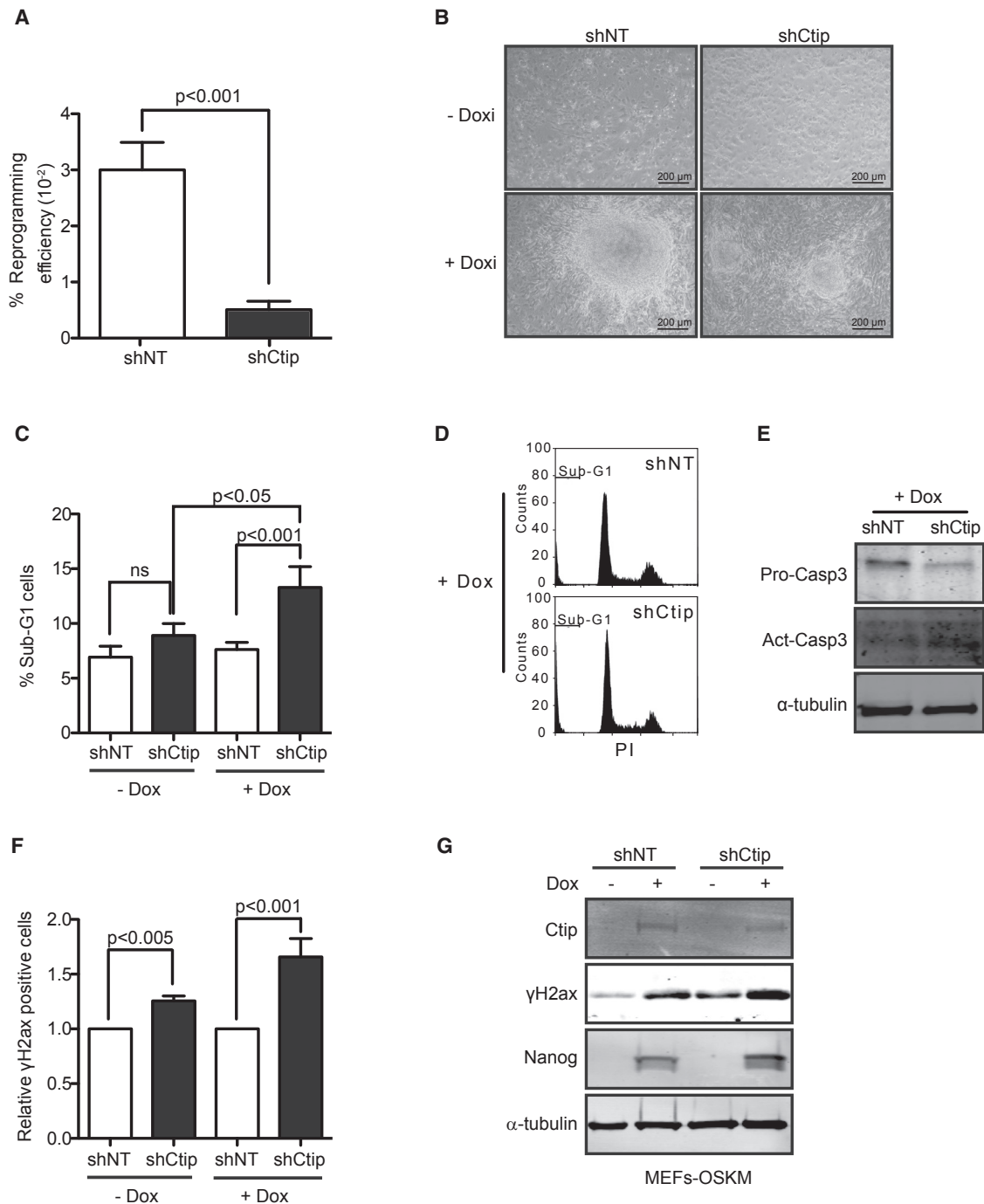
Figure 2. CtIP Deficiency Impairs Mouse Cell Reprogramming
