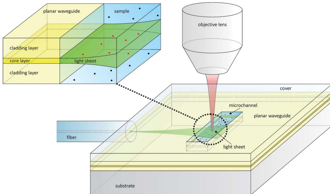
FIGURE 5 | Design of a microfluidic chip with integrated waveguide for on-chip light-sheet illumination [Figure 1 from Deschout et al. (2014)]. Laser light (green) from a fiber optic enters the planar waveguide and is confined in the vertical direction, but spreads horizontally forming a sheet of light that exits in the microchannel. The fluorescence light (red) is collected by an objective lens. The red dots show fluorophores that are excited by the light-sheet, while black dots are those that are not. Only the fluorophore molecules traversed by the light-sheet are excited, removing out of focus noise.
