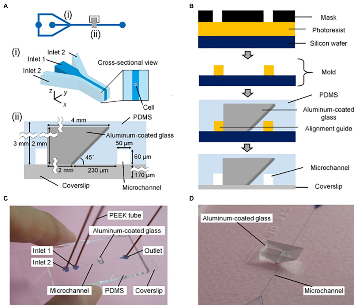
FIGURE 4 | Mirror-embedded microfluidic chip for single-objective plane illumination [Figure 3 from Miura et al. (2018)]. (A) Schematic of the channels in the microfluidic device. (i) Hydrodynamic focusing region. (ii) Optical interrogation region. (B) Diagram summarizing the microfabrication process. (C) Photograph of the microfluidic chip. (D) Close-up photograph of the microchannel and aluminum-coated reflective glass.
