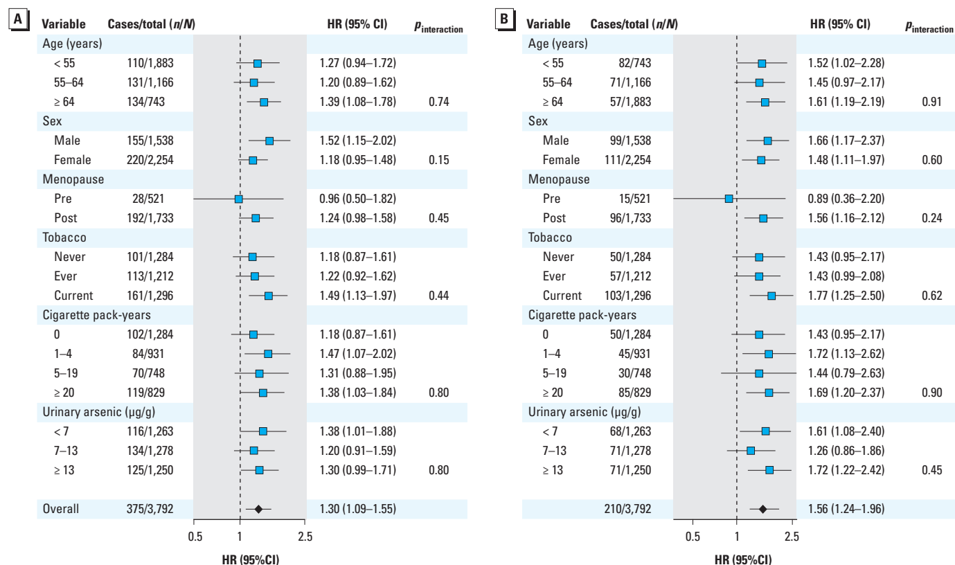
Figure 2. Fully adjusted HRs (95% CIs) for overall (A) and smoking-related (B) cancer mortality comparing the 80th versus the 20th percentile of Cd (µg/g creatinine) by participant characteristics at baseline.
