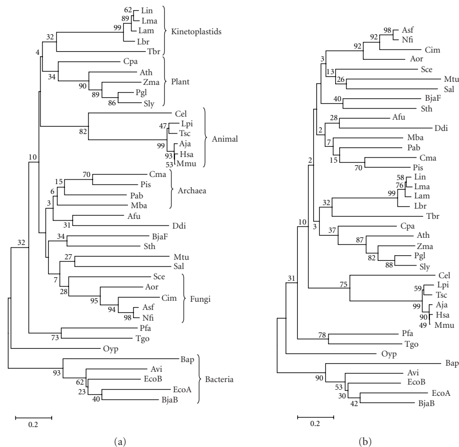
FIGURE 2: Phylogenetic analysis of sHSPs. Phylogenetic trees were constructed on the basis of \alpha -crystallin/HSP20 domains by Neighbor Joining (a) and Minimum Evolution (b) using the MEGA 3 program as described in the Material and Methods section. Sequences (UniProtKB/TrEMBL entry): Afu, Archaeoglobus fulgidus (O28308); Aja, Artibeus jamaicensis (P02482); Aor, Aspergillus oryzae (Q2TXY8); Asf, Aspergillus fumigatus (Q4WV00); Ath, Arabidopsis thaliana (O81822); Avi, Azotobacter vinelandii (P96193); Bap, Buchnera aphidicola (P57640); BjaB, Bradyrhizobium japonicum (HspB; P70918); BjaF, Bradyrhizobium japonicum (HspF; O69243); Cel, Caenorhabditis elegans (Q7JP52); Cim, Coccidioides immitis (Q1E6R4); Cma, Caldivirga maquilensis (A8MB44); Cpa, Carica papaya (Q69BI7); Ddi, Dictyostelium discoideum (Q54I91); EcoA, Escherichia coli (ibpA; P0C054); EcoB, Escherichia coli (ibpB; P0C058); Hsa, Homo sapiens (P02489); Lam, L. amazonensis ; Lbr, L. braziliensis ; Lin, L. infantum ; Lma, L. major ; Lpi, Lygodactylus picturatus (Q6EW10); Mba, Methanosarcina barkeri (Q46E59); Mmu, Macaca mulatta (P02488); Mtu, Mycobacterium tuberculosis (P0A5B7); Nfi, Neosartorya fischeri (A1DEG0); Oyp, Onion yellows phytoplasma (P81958); Pab, Pyrococcus abyssi (Q9V1L0); Pfa, Plasmodium falciparum (Q8IB02); Pis, Pyrobaculum islandicum (A1RRY3); Pgl, Picea glauca (Q40852); Sal, Streptomyces albus (Q53595); Sce, S. cerevisiae (P15992); Sly, Solanum lycopersicum (O82545); Sth, Streptococcus thermophilus (P80485); Tbr, Trypanosoma brucei (Q57V53); Tgo, Toxoplasma gondii (Q6DUA8); Tsc, Trachemys scripta (Q91517); Zma, Zea mays (P24632). The scale represents mutational changes per residue.
