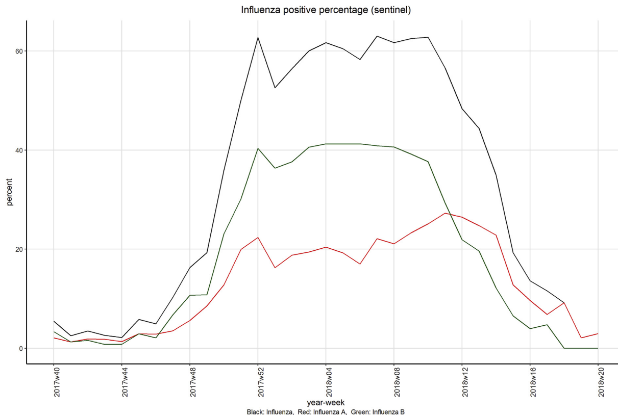
Fig. 1. Percentage influenza positive sentinel specimens, pooled from 24 European countries* by week of reporting and influenza virus type, week 40/2017 to week 20/2018.
