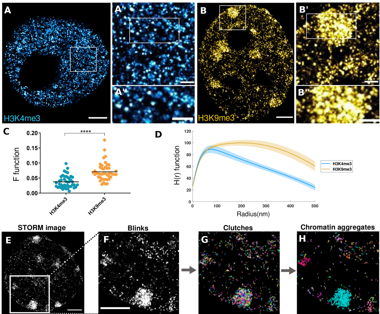
Fig. 1. Super-resolution imaging of H3K4me3 and H3K9me3 in mouse preimplantation embryos. (A,B) Representative dSTORM images of trophoctoderm nuclei from blastocyst stage embryos stained for H3K4me3 (A) and H3K9me3 (B). Progressively higher magnifications of indicated regions are shown (A',A'',B',B''). (C) Values of the F-function for all H3K4me3 (blue) and H3K9me3 (orange) labelled nuclei used in this study, where higher values indicate higher clustering levels. ****, P -value < 0.0001, t -student test. (D) H(r) function of all H3K4me3 (blue) and H3K9me3 (orange) labelled nuclei used in this study, where each function indicates the average amount of molecules that lie at distance r from a reference molecule (mean and standard error of the mean represented with lines and shadows, respectively). (E,F) dSTORM image of a blastocyst TE nucleus stained with anti-H3K9me3 and a zoom-in of the highlighted region. (G) Segmentation of the region shown in F into nucleosome clutches, shown in different colors. (H) Grouping of clutches into chromatin aggregates based on their proximity and density. Scale bars: 2 \mu m (A,B,E,F), 500 nm (A',A'',B',B'').
