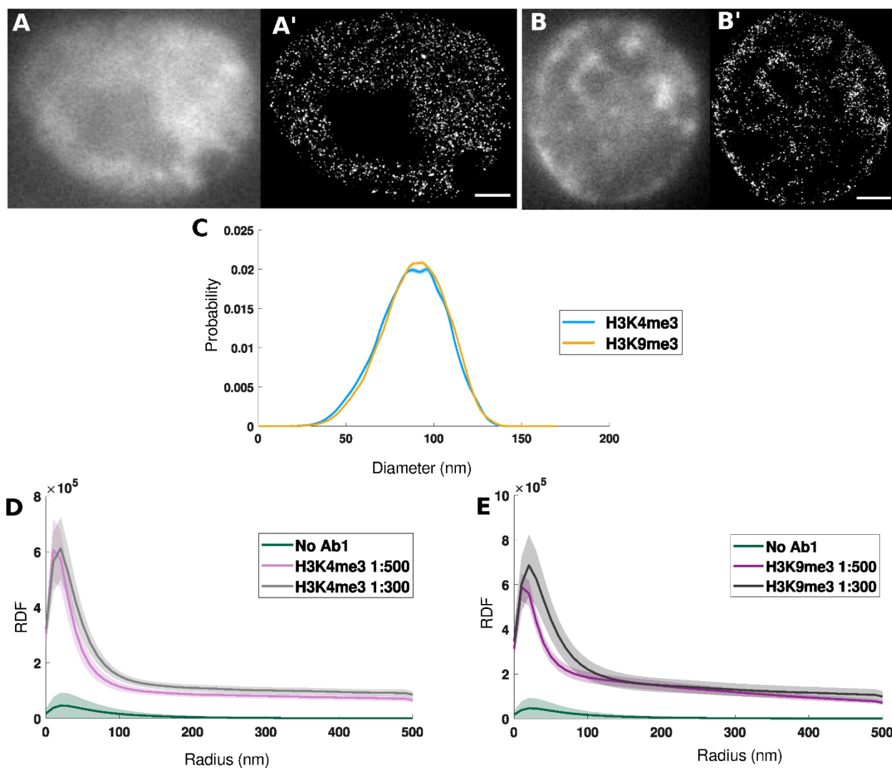
Fig. S1. d STORM enhances resolution of chromatin imaging in mouse preimplantation embryos.
