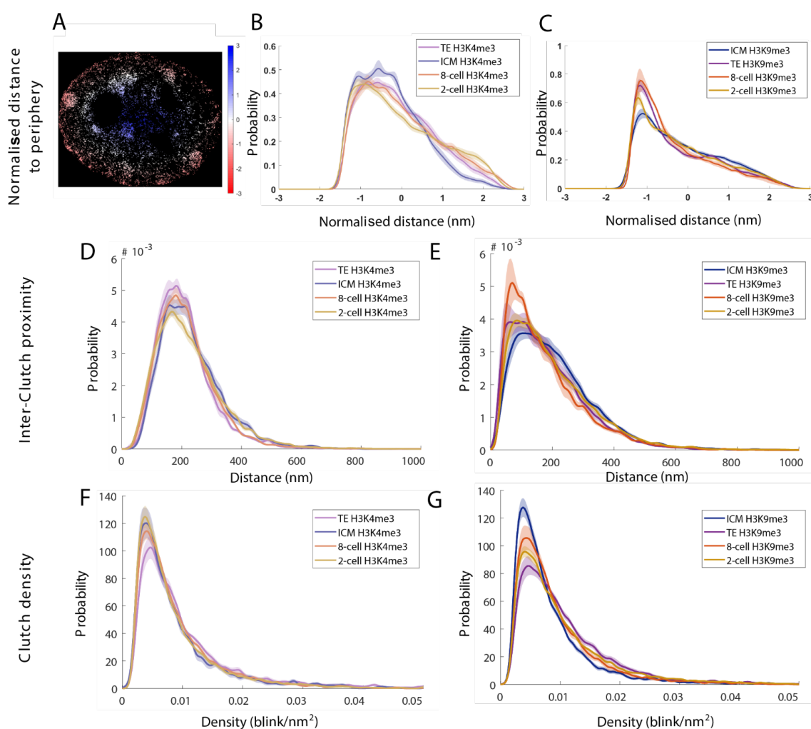
Fig. S3. Dynamics of nucleosome clutches in preimplantation development.
