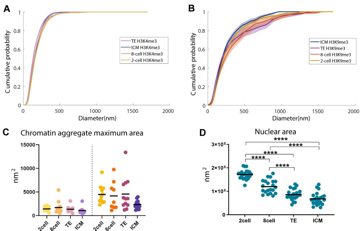
Fig. S4. Chromatin aggregates along preimplantation development.
