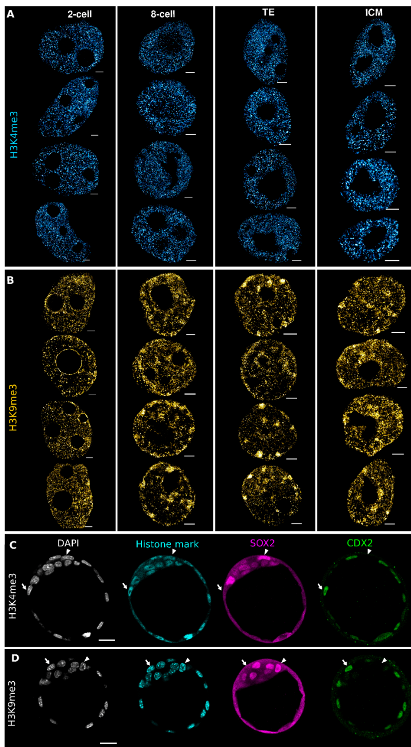
Fig. S2. dSTORM images of epigenetic marks at different developmental stages.
