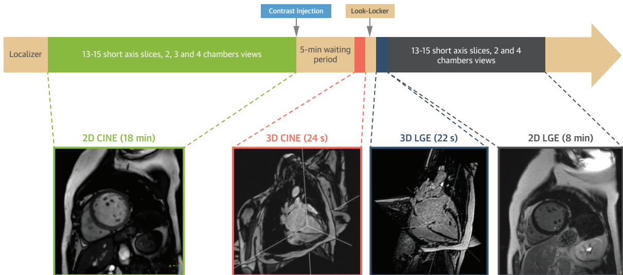
FIGURE 1 Study Design
