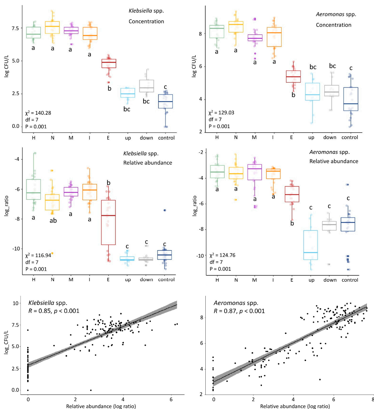
Figure 4. Comparison of colony forming units (CFU) counts and relative abundances in the different locations of Klebsiella spp. (left) and Aeromonas spp. (right). The CFU counts (log(CFU/L)) and relative abundance (log ratio) show similar patterns along the locations. This was confirmed by Pearson correlation analysis (R) shown in the linear regression curves. Kruskal-Wallis statistics of the CFU counts and relative abundances are shown on the left side of each panel: chi-squared ( \chi^2 ), df and p-value). Group differences were assessed by the Dunn's test with the p-value adjustment method: BH. The locations are shown on the horizontal axis. H = hospital, N = nursing home, C = community (municipal wastewater), I = influent, E = effluent, up = upstream surface water, down = downstream surface water, and control = surface water collected at nature reserve "de Deelen".
