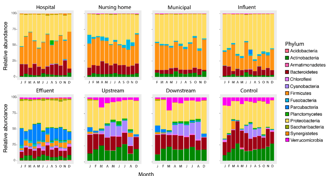
Figure 5. Relative abundance at the Phylum level per location per month. The main groups in wastewaters (hospital, nursing home, municipal wastewater and influent) consist of Proteobacteria, Firmicutes, Bacteroidetes and Actinobacter, which are significantly changed after the wastewater treatment with Proteobacteria and Parcubacteria as main groups in the effluent. Surface waters are similar to each other but form a distinct group dominated by Proteobacteria, followed by Actinobacteria and Bacteroidetes as the main Phyla.
