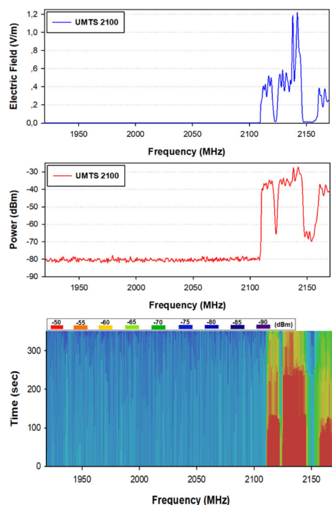
FIGURE 20. Measurement results within the tram wagon car by means of the spectrum analyzer for the UMTS 2100 frequency band: E-field values (up), Power values (middle) and spectrogram (bottom).
