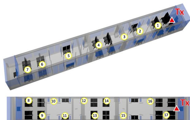
FIGURE 22. Transmitter and measurement points in the controlled measurement campaign within the tram wagon.
