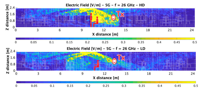
FIGURE 14. Comparison of the simulated E-field exposure levels within the tram at 26 GHz frequency band for different users' densities. The transmitter is located in the middle of the tram with 10 dBm transmitting power and a directional radiation pattern.
