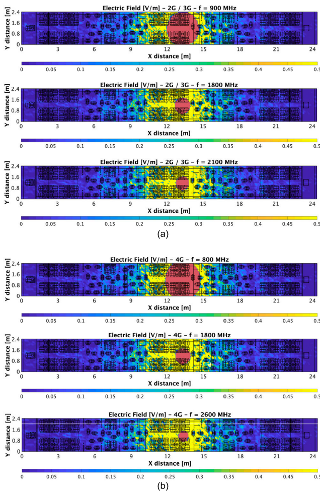
FIGURE 7. Comparison of the simulated E-field exposure levels within the tram for the high-density case. The transmitter is placed in the middle of the tram with 10 dBm transmitting power. 5 \lambda m exclusion area around the transmitter has been considered in order to avoid near field results, (a) 2G / 3G cellular systems (b) 4G cellular systems.
