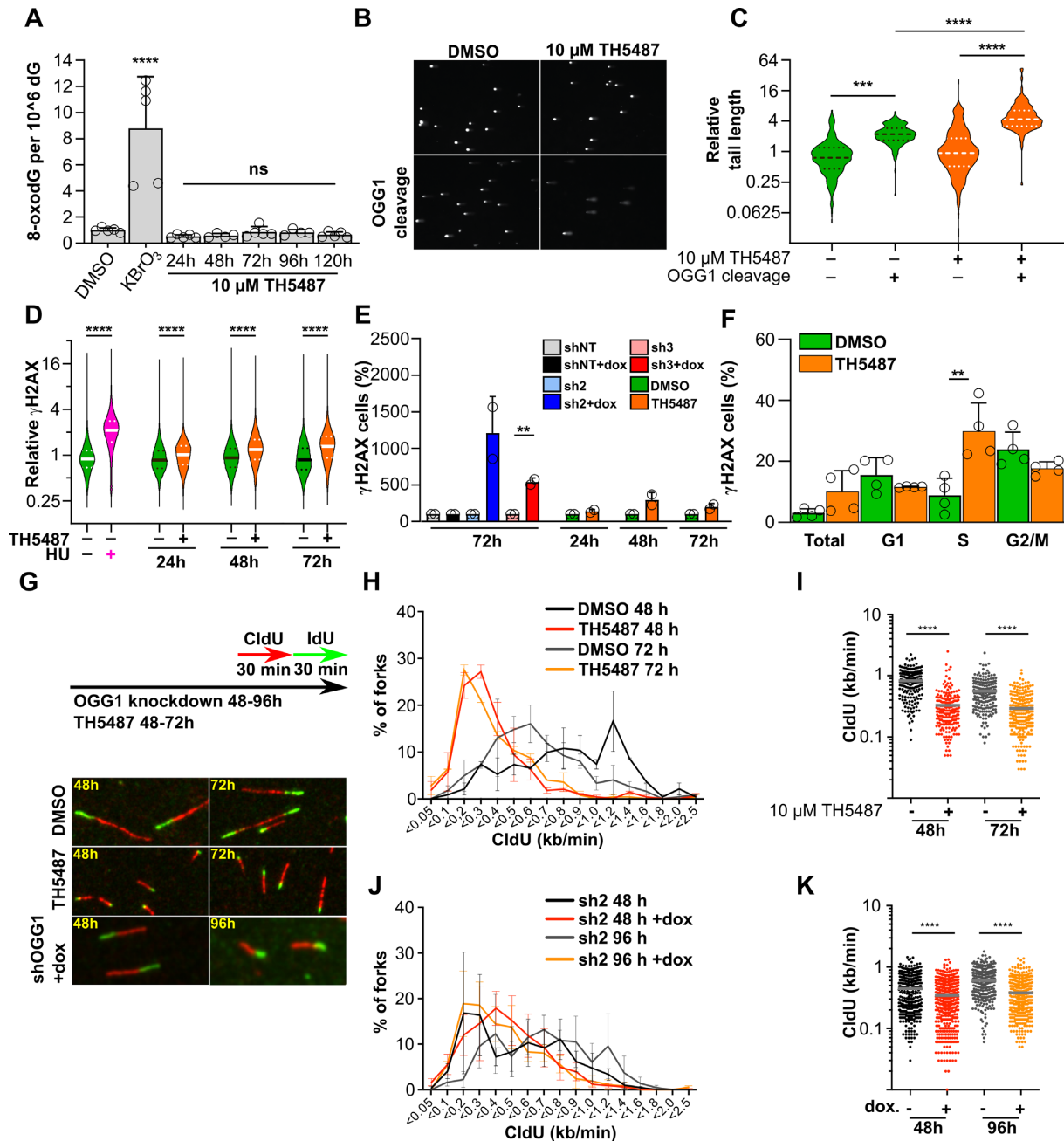
Figure 5. Effect of TH5487 on DNA lesions, DNA damage markers and DNA replication. (A) 8-oxodG accumulation in A3 cells. A3 cells were treated with 20 mM \text{KBrO}_3 for 1 h or with 10 \mu\text{M} TH5487 for the indicated times, and the amount of genomic 8-oxodG was quantified with LC-MS/MS. Data are average \pm SD of five replicates from two independent experiments. (B) Comet assay. A3 cells were treated with 10 \mu\text{M} TH5487 for 72 h and strand-breaks and OGG1 substrate lesions were analyzed with the OGG1-modified Comet assay. Representative images of cells are shown. (C) Violin blot of Comet tail moment. Cells were treated as in B, and the tail moment of the cells were analyzed using blinded automatic analysis ( n = 200 per condition from two independent experiments). The full line indicates median, and the dotted lines quartiles. (D) Violin blot of phosphorylated \gamma\text{H2AX} intensity. A3 cells were treated with 0.1% DMSO or 10 \mu\text{M} TH5487 for the indicated times and stained for phosphorylated \gamma\text{H2AX} . Treatment with 2 mM Hydroxyurea for 1 h was used as positive control. At least 33 000 nuclei per group were quantified from three independent experiments. The full line indicates median, and the dotted lines quartiles. All values are normalized to that of the mean value of the 1 h non-treated sample. (E) Relative induction of positive \gamma\text{H2AX} cells in OGG1 shRNA depleted cells for 72 h or OGG1 inhibited with 10 \mu\text{M} of TH5487 for 24, 48 and 72 h. Data are average \pm SD of two technical replicates representative of 1–2 independent experiments (F) Relative cell cycle distribution of positive \gamma\text{H2AX} gated cells along G1, S or G2/M cell cycle phases after 72 h treatment with 10 \mu\text{M} TH5487. Data are average \pm SD of two technical replicates from two independent experiments. (G) Experimental setup of DNA fiber assay. A3 cells were treated with 0.1% DMSO or 10 \mu\text{M} TH5487 for 48 h or 72 h, alternatively A3 shOGG1#2 were treated with doxycycline for 48 or 96 h followed by addition of 5-chloro-2'-deoxyuridine (CldU) or 5-iodo-2'-deoxyuridine (IdU) to the medium. Representative images of DNA replication fibers are shown. (H) Distribution of fork speed in CldU-labelled A3 cells treated with DMSO or TH5487 for 48 or 72 h. (I) Total fork speed in DMSO and TH5487-treated cells. (J) Distribution of fork speed in CldU-labelled A3 shOGG1#2 cells treated or not with doxycycline. Data shown as average \pm SD from three independent experiments. At least 300 forks were scored per condition. Statistical significance was determined using unpaired, two-sided t -tests (** P < 0.01 , *** P < 0.001 and **** P < 0.0001 ; ns, non-significant).
