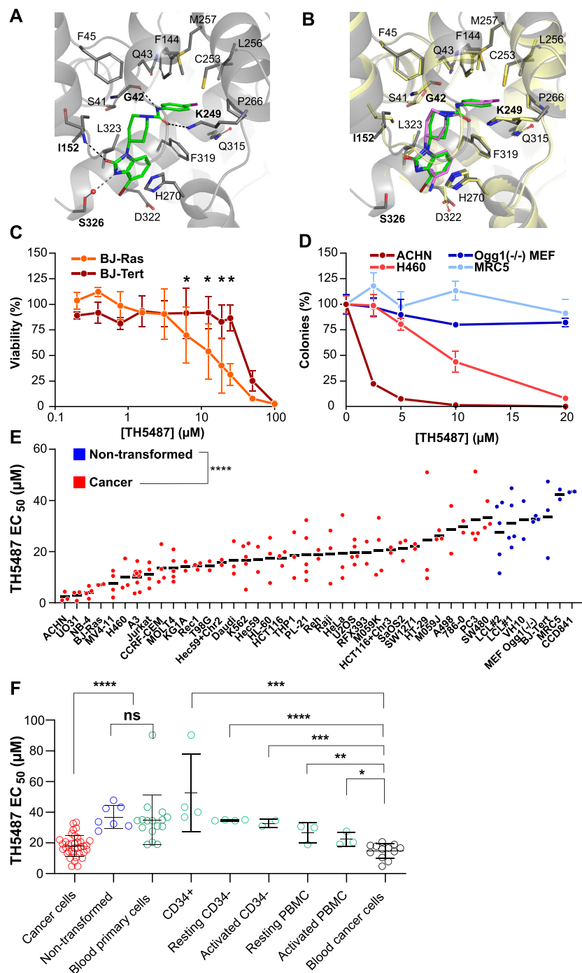
Figure 3. The OGG1 inhibitor TH5487 is selectively toxic to oncogene-expressing cells and cancer cell lines. (A) Close-up view of ligand TH5487 (green) binding to human OGG1. Important residues in the binding site are marked, hydrogen bond interactions are shown in black dashed line, water (red sphere)-mediated interactions in grey dashed line. (B) Comparison between the binding of ligand TH5487 (green) to human OGG1 (gray) with the structure of TH5675 (pink) bound to mouse OGG1 (yellow, PDB 6G3Y). (C) Viability of BJ-Tert and BJ-Ras cells exposed to the indicated concentrations TH5487 for five days. Data are average \pm SD of four technical replicates from two independent experiments. (D) Clonogenic survival of cell lines exposed to TH5487. The cancer cell lines ACHN and H460, and the non-transformed cell lines MRC5 and Ogg1 -/- mouse embryonic fibroblasts (MEF) were incubated for 6–11 days in the presence of the indicated concentrations TH5487, followed by colony enumeration. Data are average \pm SD values of four technical replicates, representative of three independent experiments. (E) TH5487 selectively decreases viability of cancer cell lines. EC 50 -values of 34 cancer (red) and 7 non-transformed cell lines (blue). Cells were exposed to a dilution series of TH5487 for five days followed by a viability assessment using resazurin. All cell lines were tested in two to ten independent experiments. Each point represents the EC 50 -value from one experiment (average of two or three technical replicates). (F) Comparative analysis of EC 50 values for TH5487 in cancer- and non-transformed cell lines, and CD34+ hematopoietic stem cells, CD34-fraction from cord blood or PBMCs from healthy donor blood. All primary blood cells were tested upon activation with Dynabeads/Phytohemagglutinin or not and exposed to a dilution series of TH5487 to calculate EC 50 values by resazurin assay. Data for blood cells are average \pm SD from two to four independent donors, and are significantly different from the hematological cancer cell lines tested, using a two-sided unpaired t -test (* P < 0.05, ** P < 0.01, *** P < 0.001 and **** P < 0.0001, ns, non-significant).
