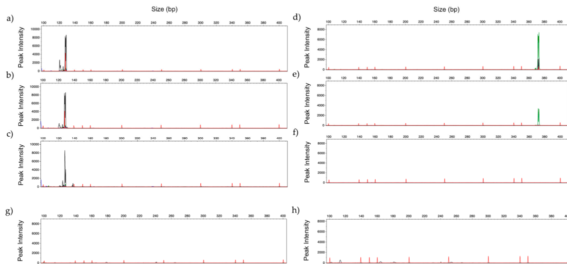
Figure 4. GeneScan profiles obtained by multiplex analysis testing: (a) 100 pg; (b) 10 pg and (c) 1 pg of DNA of C. glabrata (black) with Candida Panel, and (d) 100 pg; (e) 10 pg and (f) 1 pg of DNA of A. flavus (green) with Filamentous Fungi Panel. (g,h) represent the multiplex profile with 486 ng of commercial human DNA, with Candida Panel and Filamentous Fungi Panel, respectively. (Fluorescent dyes HEX = green, NED = black).
