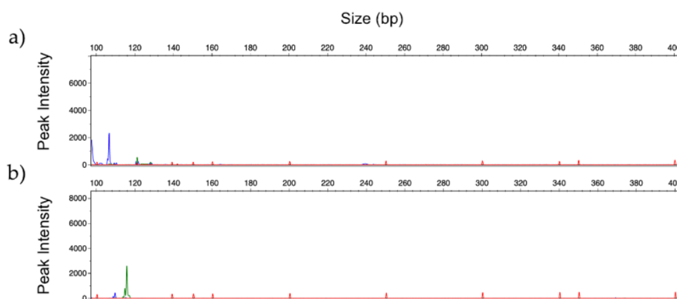
Figure 7. GeneScan profiles obtained by multiplex analysis of clinical samples identified as: (a) C. albicans (blue) and (b) A. fumigatus (green), using Candida Panel and Filamentous Fungi Panel, respectively. (Fluorescent dyes FAM = blue, HEX = green).
