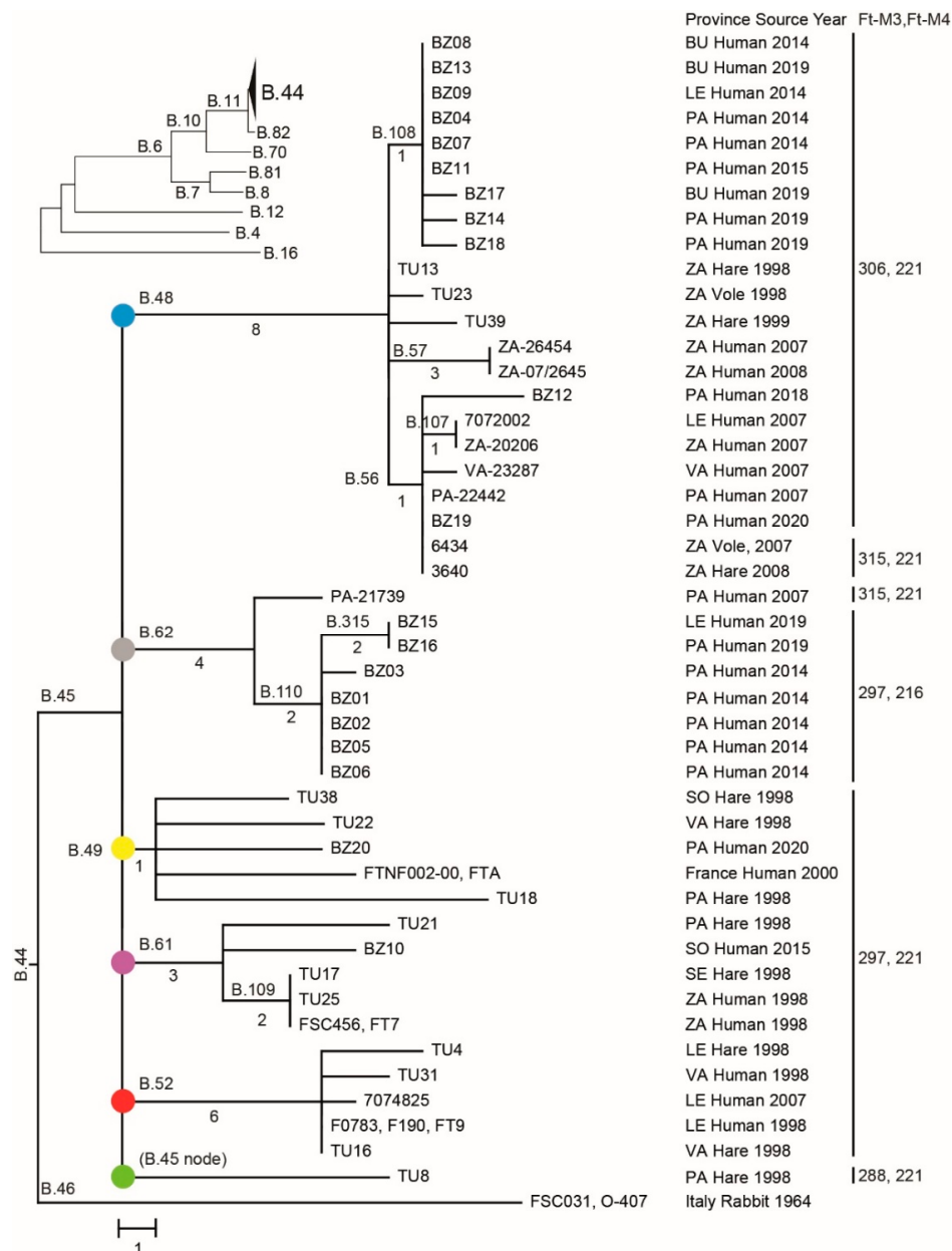
Figure 1. Neighbor-joining phylogeny based on 117 single-nucleotide polymorphisms (SNPs) in whole-genome sequencing (WGS) data of 45 F. tularensis strains from Spain, 1998 to 2020, and two reference genomes from France and Italy demonstrating a star-like branching pattern. The tree is rooted in the Italian genome as this genome is the most ancestral in relation to the global Francisella tularensis subspecies holarctica phylogeny (see the upper-left inset tree). Major genetic groups of strains from Spain are labelled by color-filled circles. Tree branches are labelled by canSNPs (the letter B followed by a number). The number of SNPs along the branches is indicated for branches with multiple taxa (see Appendix A Table A4 for canSNP positions in the reference strain FTNF002-00). Province abbreviations are Burgos (BU), León (LE), Palencia (PA), Segovia (SE), Soria (SO), Valladolid (VA), and Zamora (ZA). Variable-number tandem repeat (VNTR) marker data are in the right column.
