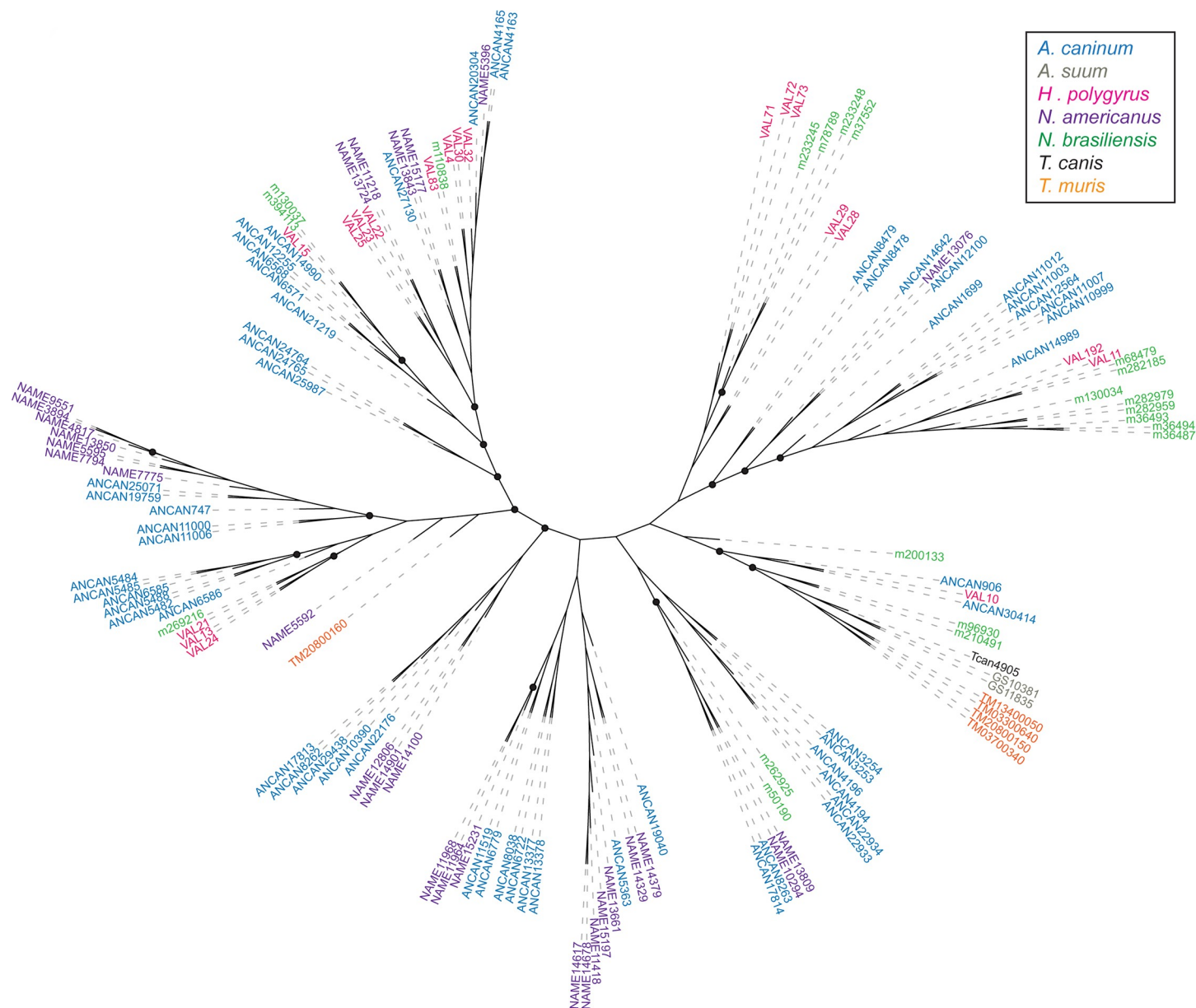
Fig 6. Phylogenetic relationships of single-domain SCP/TAPS proteins determined with MUSCLE alignment software. PhyML was used for a maximum-likelihood phylogenetic analysis with bootstrapping and results were visualized with The Interactive Tree of Life (iTOL) online phylogeny tool. Necator americanus sequences are highlighted in purple with comparator species each denoted by a different color (see key). Black solid circles on branches denote bootstrap values greater than or equal to 70% support.
