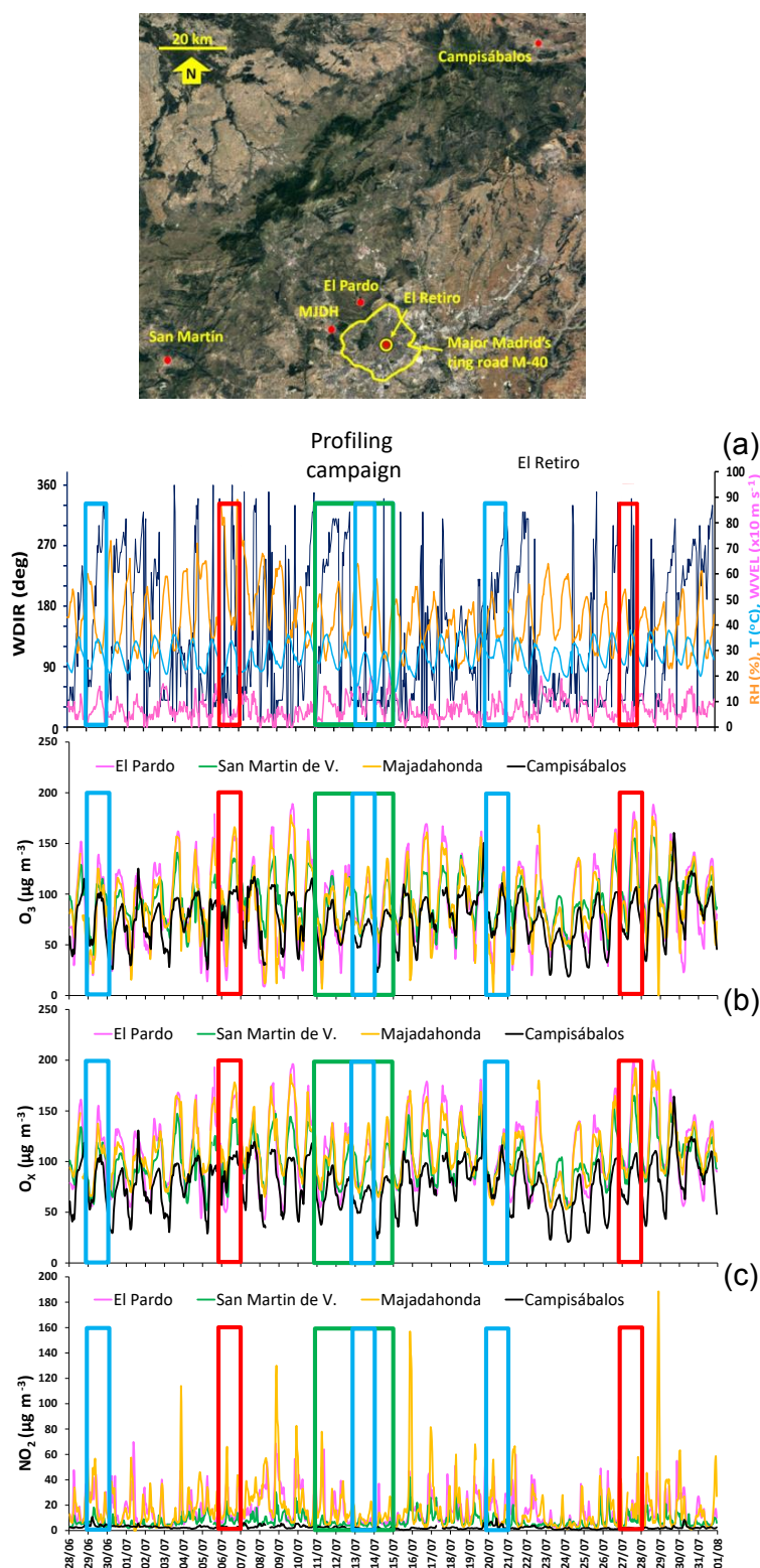
Figure 2. (a) Hourly meteorological parameters recorded at El Retiro air quality monitoring station in central Madrid (from 28 June 2016 to 1 August 2016). (b) Hourly concentrations of \text{O}_3 and \text{O}_x ( \text{O}_3 + \text{NO}_2 ) recorded at a selection of air quality monitoring stations representing the greater Madrid area, together with those from the remote background station of Campisábalos. (c) Hourly \text{NO}_2 concentrations recorded at the same sites for the same period. Periods with available AEMET free soundings of \text{O}_3 are bracketed with red (accumulation) or blue (venting) squares. The vertical \text{O}_3 and UFP profiling campaign is marked with a green square.
