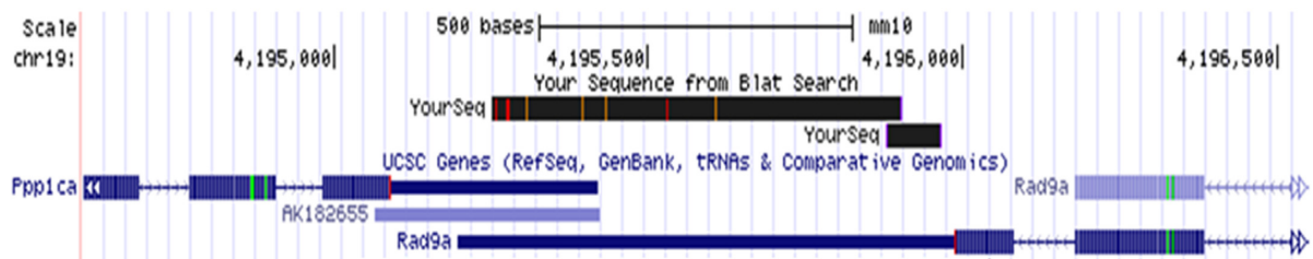
Figure 1. A putative chimera composed of RAD9A (RAD9A homolog A) and PPP1CA (protein phosphatase 1). (A) A chimera found among human ESTs. (B) A mouse chimera.
